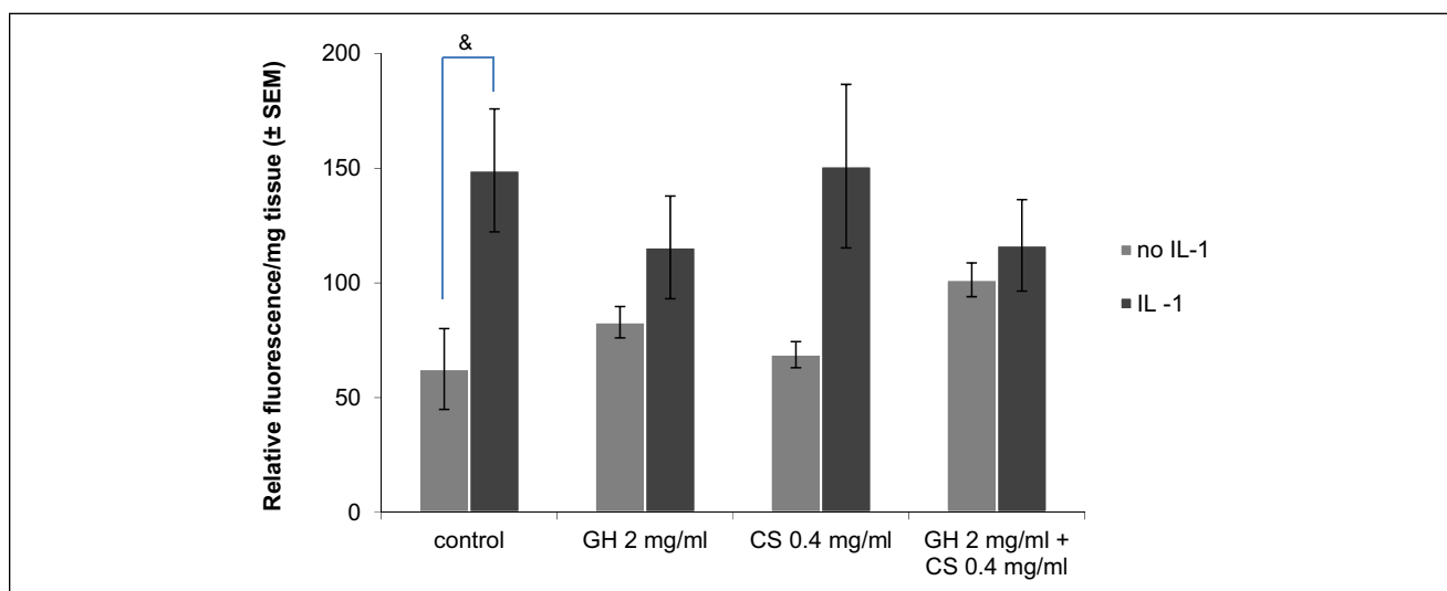
Figure 5. Effect of glucosamine hydrochloride (GH) and chondroitin sulfate (CS) on ADAMTS-4 activity at 72 hours post-stimulation with interleukin-1 \alpha (IL-1 \alpha ). Values represent the mean relative fluorescence per mg tissue \pm SEM, n = 3. One-sample Student t test was used. & indicates P < 0.05 for comparison between no-IL-1 \alpha and IL-1 \alpha control samples.
