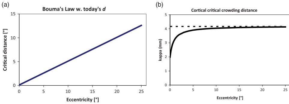
Figure 17. (A) Bouma's law in the visual field and (B) its cortical equivalent, that is, how it translates to the cortical map in a primary visual area (Strasburger, 2019, Figure 8; see there for the specific parameters chosen for the estimation and note that kappa depends upon these).
