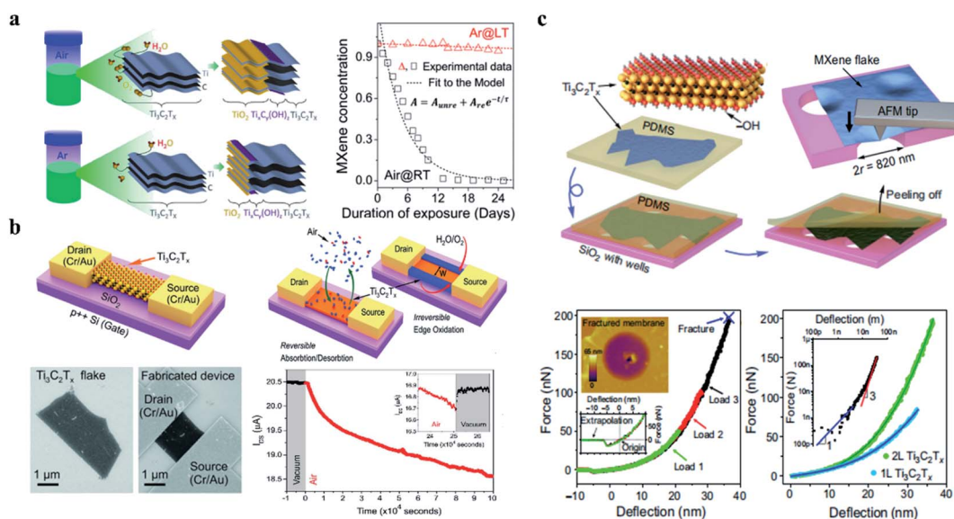
Fig. 3 (a) Oxidation process and rate of Ti_3C_2T_x MXene dispersion in air and argon. 34 (b) The schematic diagram of an electrical performance measurement device based on Ti_3C_2T_x MXene. 41 (c) The measurement method and process diagram of Young's modulus of Ti_3C_2T_x MXene. 44
