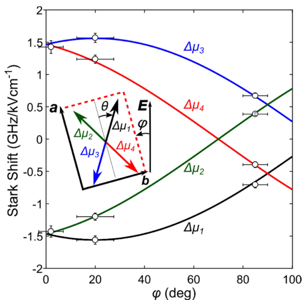
Figure 5. Angle-dependent Stark shift as a function of the angle, \varphi , between the crystallographic axis and the electric field. The Stark shift is calculated for four electric dipoles (rotated by -\theta + \varphi , \theta + \varphi , \pi - \theta + \varphi , \pi + \theta + \varphi and compared to the experimental data (hollow circles). The simulated values are determined for the maximum of the Stark shift 1.56 \pm 0.06 GHz/ \text{kVcm}^{-1} and \theta = 20^\circ . The inset illustrates the orientation of the four dipoles used in calculation; a and b axes, electric field vector E , as well as angles \theta and \varphi are shown.
