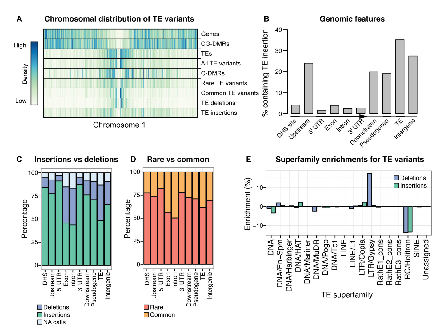
Figure 2. Extensive novel genetic diversity uncovered by TE variant analysis. (A) Distribution of identified TE variants on chromosome 1, with distributions of all Col-0 genes, Col-0 TEs, and population DMRs. (B) Proportion of different genomic features containing one or more TE variants. (C) Proportion of TE variants within each genomic feature classified as deletions or insertions. (D) Proportion of TE variants within each genomic feature classified as rare (<3% MAF) or common (≥3% MAF). (E) Enrichment and depletion of TE variants categorized by TE superfamily compared to the expected frequency due to genomic occurrence.
