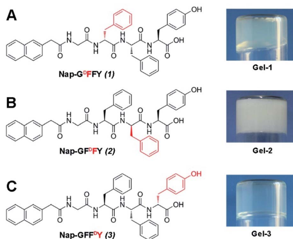
Fig. 1 The chemical structures and optical images of (A) Nap-G D FFY, (B) Nap-G D D FFY and (C) Nap-G D D D FFY hydrogels.
