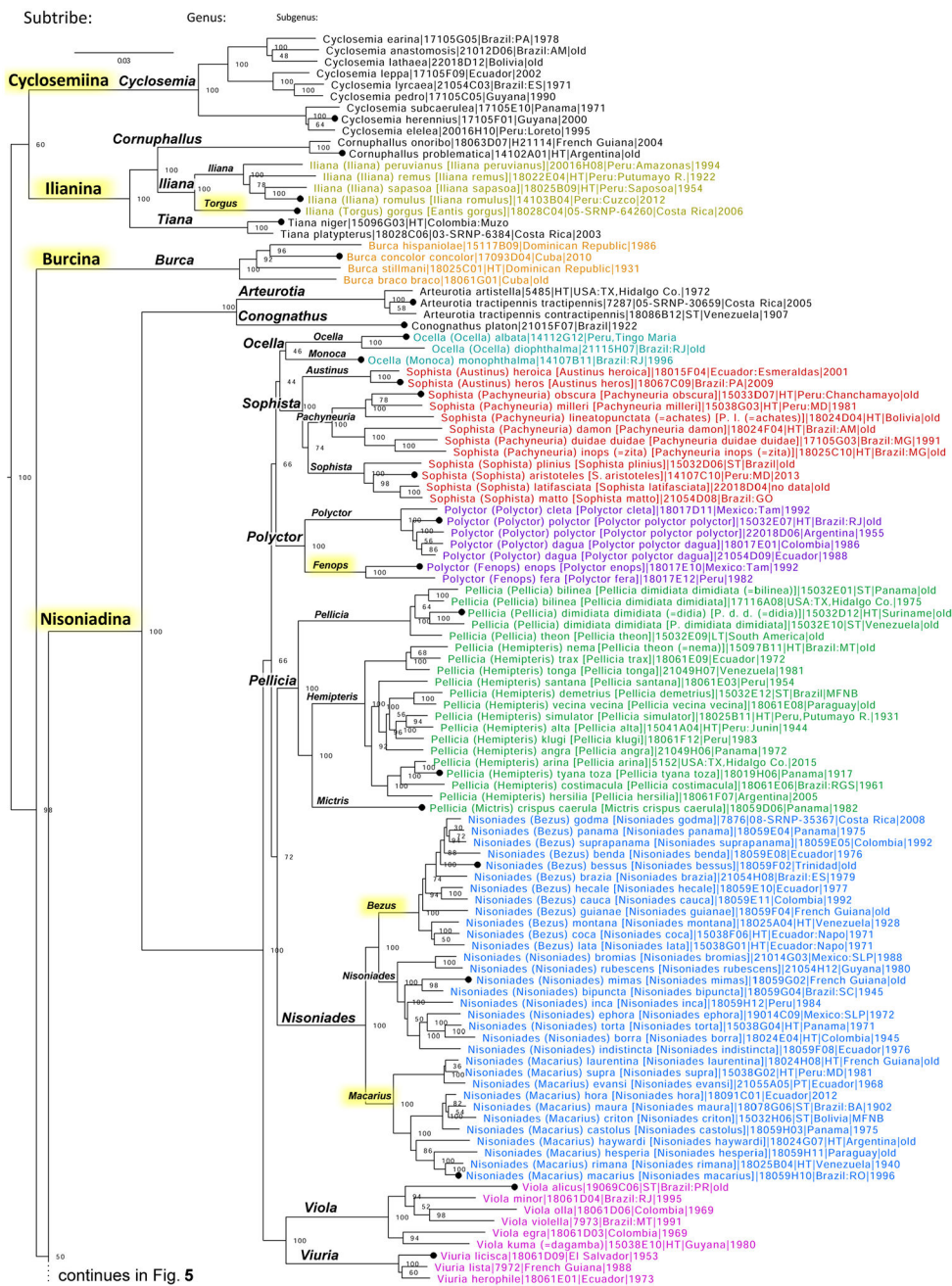
Figure 4. The nuclear genome-based phylogeny of Carcharodini, first segment (continues in Fig. 5, 6). See Fig. 1 for notations.
