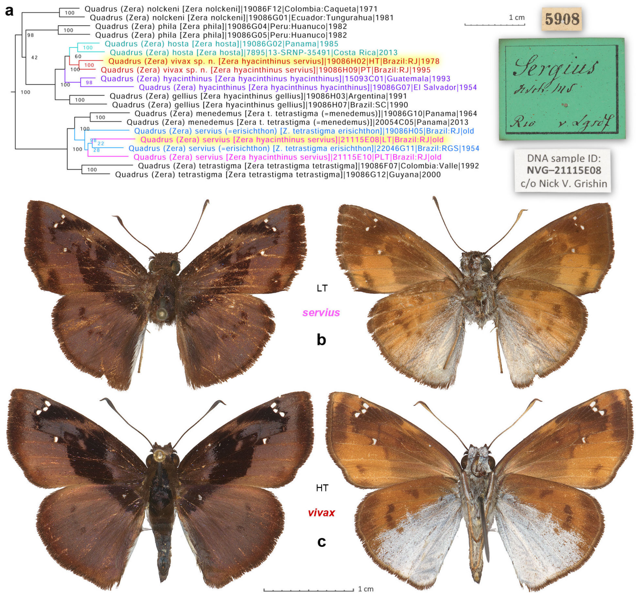
Figure 2. Quadrus (Zera) nuclear genome-based phylogeny and type specimens. a ) The nuclear genome-based phylogeny of selected species: Q. vivax sp. n. (red), Q. hyacinthinus (purple), Q. hosta (cyan), Q. servius stat. rest. (blue and magenta, with its synonym Achlyodes erisichthon labeled in blue) rooted with the remaining Zera species (not shown; see Fig. 1). Specimens shown below are highlighted in yellow; see Fig. 1 for other notations. b ) Lectotype of Quadrus (Zera) servius designated herein, with its labels shown above on the right. c ) Holotype of Quadrus (Zera) vivax sp. n. Specimens are in dorsal (left) and ventral (right) views, data in text. The scale bar at the bottom refers to specimens; the scale bar at the top refers to labels reduced by 1/3 compared to specimens.
