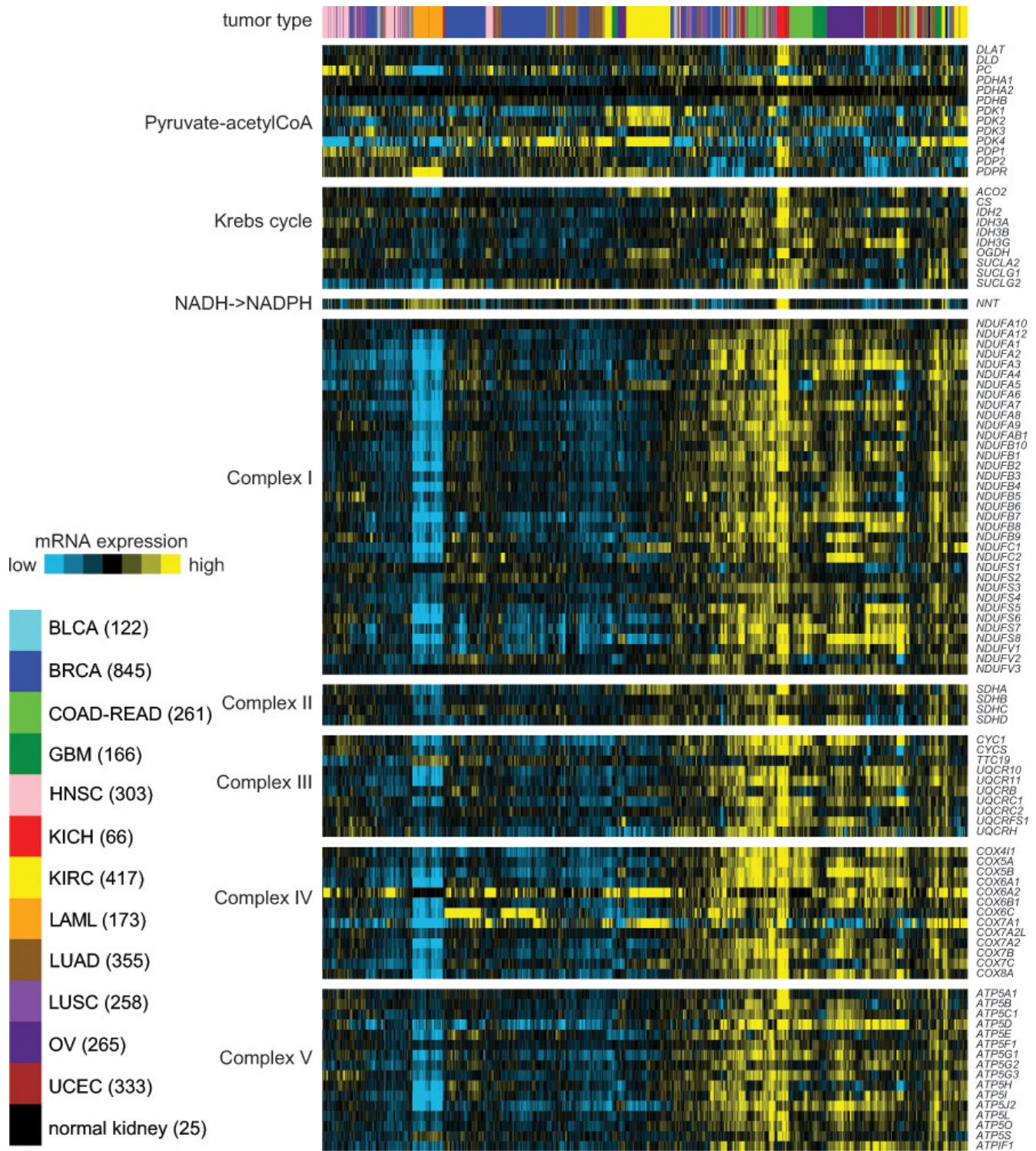
Figure 1: In a panel of human cancers of various tissues of origin (from TCGA, n = 3,564 samples), differential expression (relative to sample median) of genes related to Krebs cycle and Electron Transport Chain (ETC). RNA-seq profiles are from the recent TCGA pan-cancer multiplatform subtyping analysis, with the addition of sample profiles of ChRCC (KICH) and normal kidney from TCGA ChRCC study [1]. On the basis of the expression patterns of the selected genes, samples were clustered by unsupervised hierarchical method [50]. KICH, chromophobe renal cell carcinoma (ChRCC); BLCA, bladder cancer; BRCA, breast cancer; COAD, colon cancer; GBM, glioblastoma; HNSC, head and neck squamous cell carcinoma; KIRC, clear cell renal cell carcinoma (ccRCC); LAML, acute myeloid leukemia; LUAD, lung adenocarcinoma; LUSC, lung squamous; OV, serous ovarian cancer; READ, rectal cancer; UCEC, endometrial cancer.
