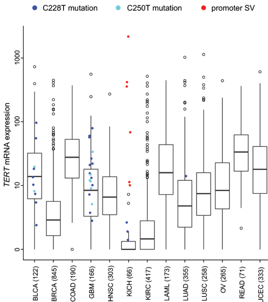
Figure 2: In a panel of human cancers of various tissues of origin (from TCGA, n = 3,564 samples), TERT mRNA expression levels by cancer type. Also indicated are those cases previously found to harbor a TERT promoter mutation (C228T or C250T) by WGS analysis (n=555 human tumors)[1, 46], as well as the ChRCC (KICH) cases for which a structural variant (SV) breakpoint within the TERT promoter region was found [1]. For Box plots, boxes represent 25% (Q1), median, and 75% (Q3), and the upper whisker is the most extreme value that is no more than Q3+1.5 IQR and the lower whisker is the most extreme value that is no less than Q1-1.5 IQR. See Figure 1 legend for tumor type designations.
