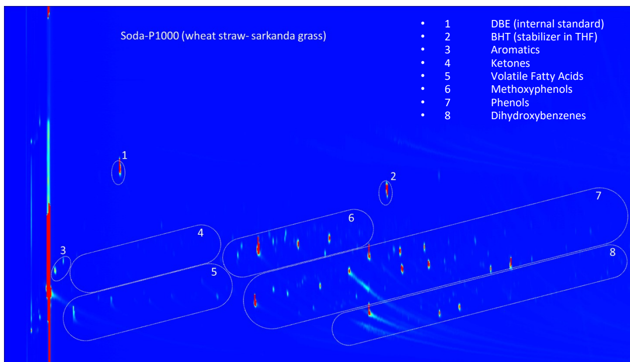
Figure S2. GC×GC chromatogram of the lignin oil obtained by BCD of Soda-P1000
