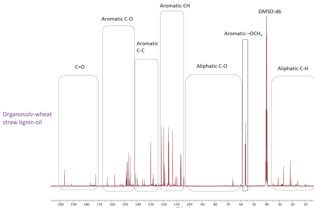
Figure S14. 13 C NMR Organosolv wheat straw lignin oil obtained by BCD
