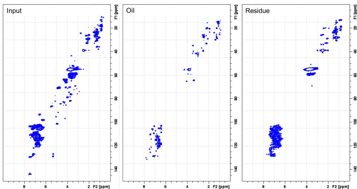
Figure S11. ^1\text{H} - ^{13}\text{C} HSQC NMR spectra of organosolv wheat straw lignin oil obtained by base catalysed depolymerisation
