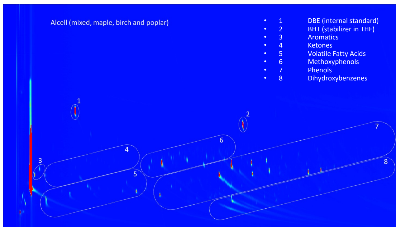
Figure S4. GCxGC chromatogram of the lignin oil obtained by BCD of Organosolv alcell
