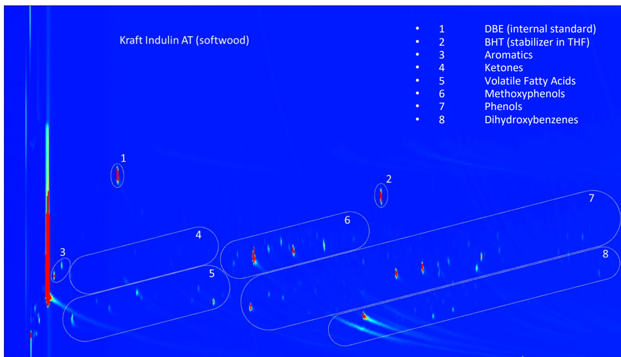
Figure S3. GC×GC chromatogram of the lignin oil obtained by BCD of Kraft Indulin AT
