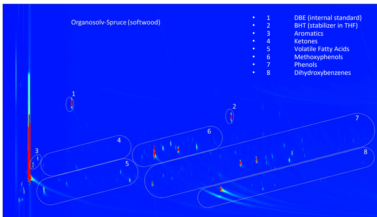
Figure S5. GCxGC chromatogram of the lignin oil obtained by BCD of Organosolv spruce
