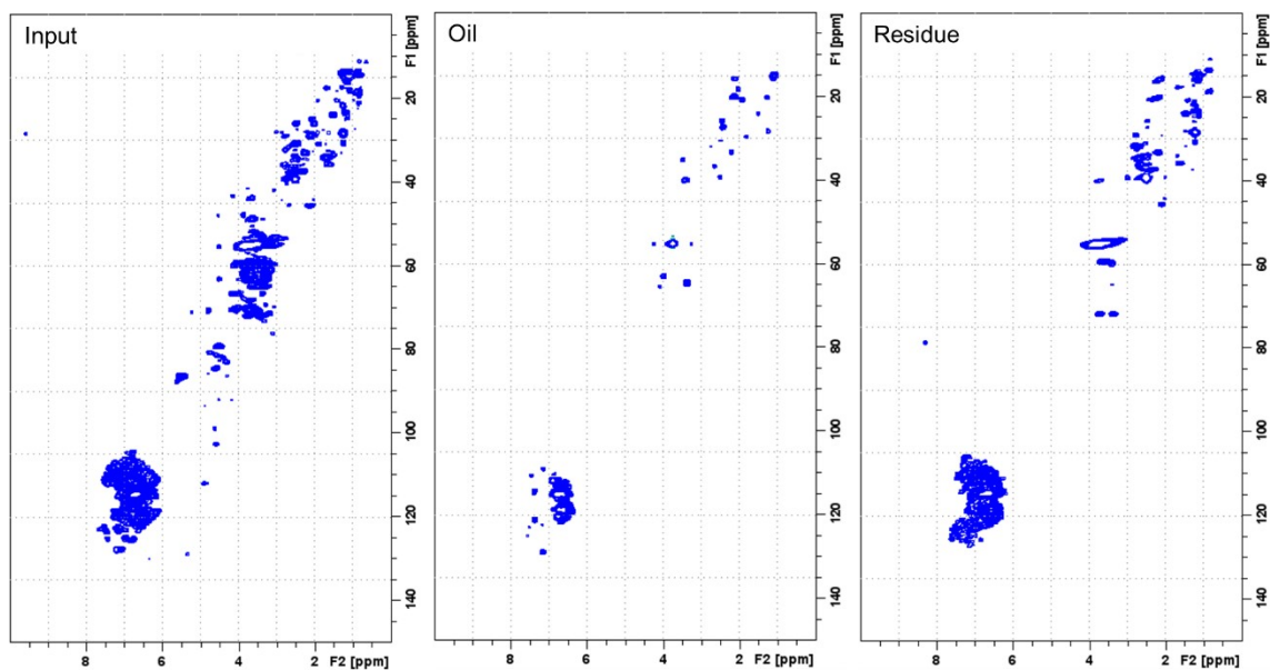
Figure S10. ^1\text{H} - ^{13}\text{C} HSQC NMR spectra of organosolv softwood spruce lignin oil obtained by base catalysed depolymerisation
