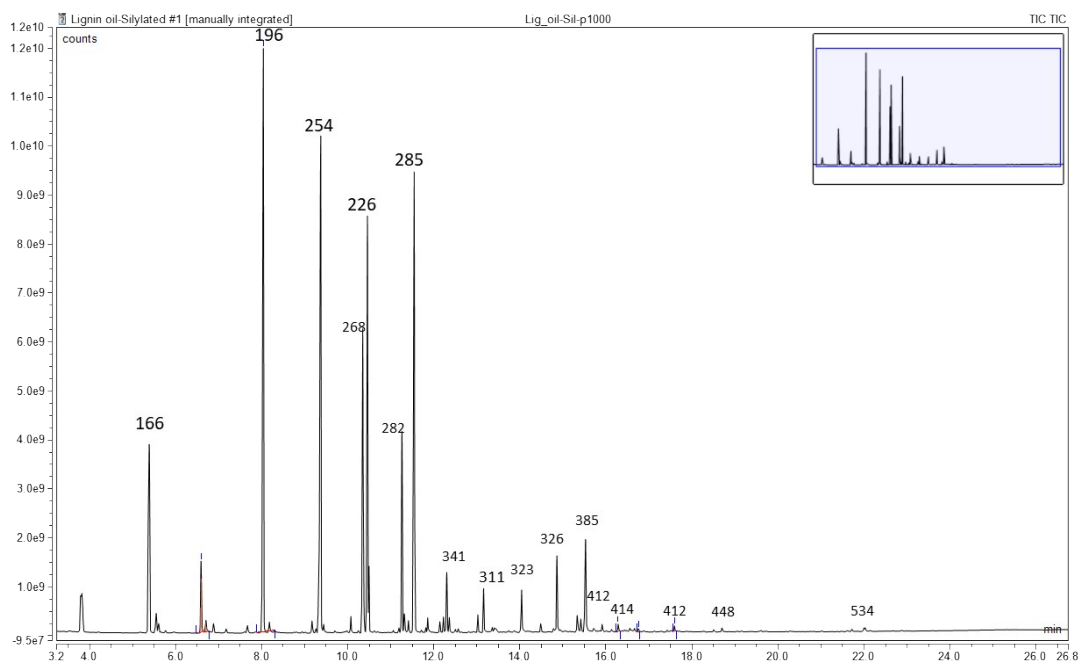
Figure S15: Typical GC-MS (after silylation) chromatogram of lignin oil (P1000) obtained by BCD. m/z values are provided on the top of each peak
