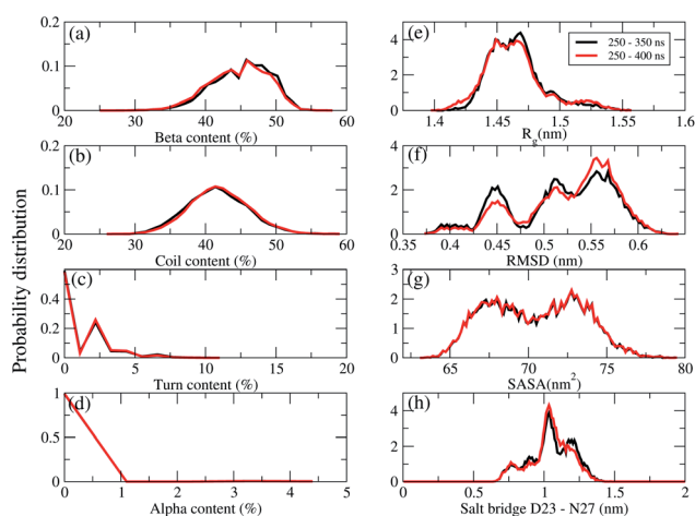
Fig. 3 REMD simulations convergence at 324 K. Probability distributions (unnormalized) of the secondary structures (a) beta, (b) coil, (c) turn, (d) alpha contents, (e) the radius of gyration ( R_g ), (f) the RMSD, (g) the total solvent-accessible surface area, (h) the salt bridge D23–N27 of chain A of the transmembrane F19W 3A\beta_{11-40} . The results were calculated for two time windows 250–350 ns (black curves) and 250–400 ns (red curves).
