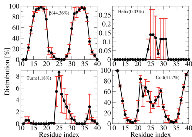
Fig. 4 Secondary structure distributions per residue averaged for all three chains of the transmembrane F19W 3A\beta_{11-40} . For clarity, the distribution of each secondary structure is presented on a different scale. The average values are given in the parenthesis.
