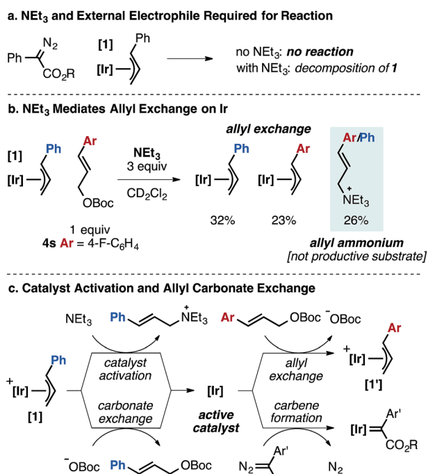
Fig. 3 Mechanistic aspects of the Ir-catalyzed cross-coupling of \alpha -aryl diazo esters and allylic carbonates based on stoichiometric reactions (steps drawn as irreversible for clarity).
