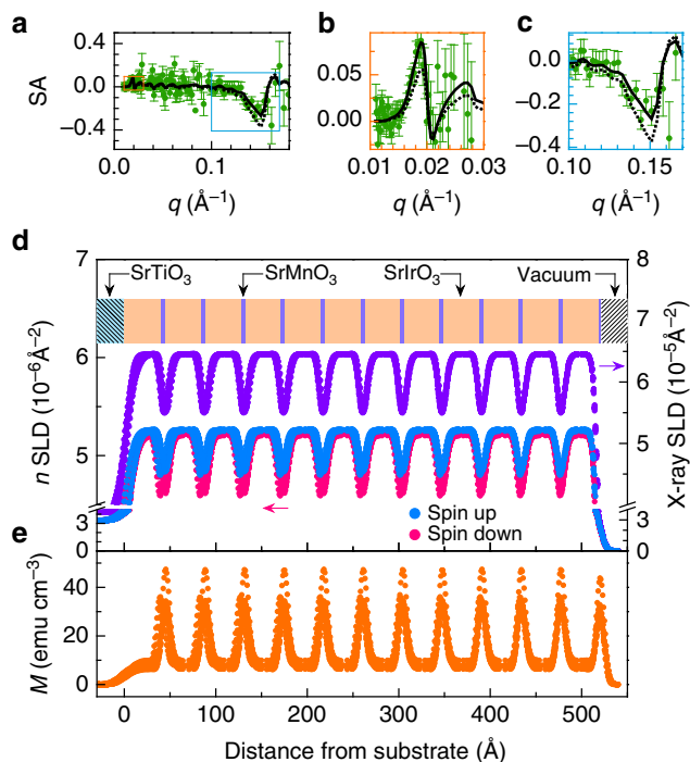
Figure 3 | Magnetic depth profiling by PNR. Data were obtained from a [(SrMnO 3 ) 1 /(SrIrO 3 ) 10 ] 12 superlattice on STO after a zero-field cooling at T = 10 K and H = 11.5 kOe with H \perp c . (a) The spin asymmetry ( SA = [R_{\uparrow} - R_{\downarrow}] / [R_{\uparrow} + R_{\downarrow}] ), where solid (dotted) black lines represent models where the magnetism in the SIO layer is allowed to vary (forced to zero) for the fit. The orange and cyan rectangles represent the positions near the critical angle and first superlattice Bragg reflection shown in b and c , respectively. (d) Depth profile of X-ray (purple) and neutron (blue and pink) scattering length densities, where a schematic drawing of the sample geometry is shown above the data. (e) Magnetic depth profile obtained with fit parameters of M_{Mn} = 85 emu cm -3 (0.54 \mu_B /Mn) and M_{Ir} = 9 emu cm -3 (0.06 \mu_B /Ir).
