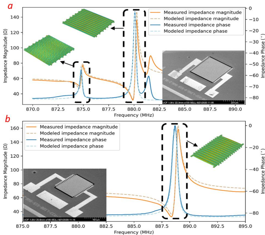
Figure 3. The measured and modeled impedance magnitude and phase of MEMS#1 (a) and MEMS#2 (b) resonators used in the sensor with the mode shapes (as simulated using COMSOL) corresponding to (a) 874.7 MHz and 879.9 MHz and (b) 888 MHz modes placed as insets.
