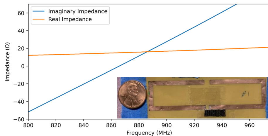
Figure 6. Real and imaginary impedances of the final antenna design with the fabricated antenna inserted as inset.
