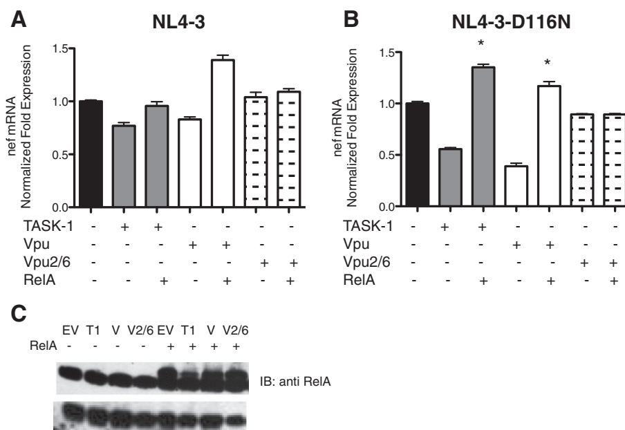
Figure 7 Suppression of HIV-1 transcription by Vpu and TASK-1 is abrogated by HIV-1 overexpression of RelA. Jurkat cells were transfected with EV, TASK-1 or Vpu or EV + RelA, TASK-1 + RelA or Vpu + RelA and then infected with wildtype NL4-3CFP (A) or NL4-3-D116N-YFP (B). Twenty four hours after infection the cells were lysed and total RNA was isolated and used as template for real-time PCR to measure nef mRNA. Data shown are normalized to empty vector control (C). Transfected Jurkat cells were harvested, lysed and equal amounts of lysate protein were subjected to 4-12% SDS-PAGE. After transfer to nitrocellulose membranes, Vpu, RelA and \beta -tubulin proteins were revealed by immunoblotting with polyclonal antibodies and visualized by chemiluminescence detection. (* P < .0001 ; Student T test was used to determine statistical significance).
