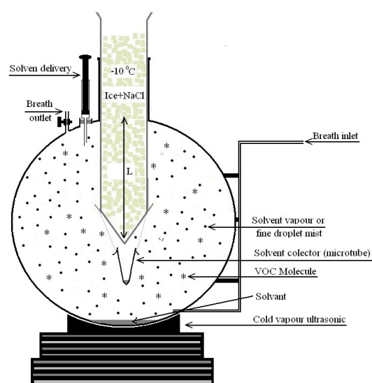
Fig. 1. Schematic presentation of designed and home-made sampling and co-liquefaction device.
