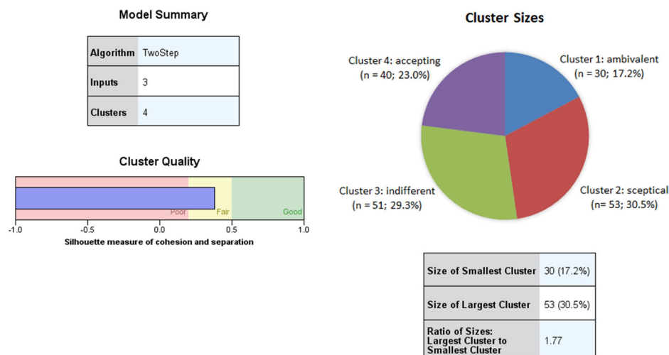
Figure 1 Test statistics of clustering analysis.
