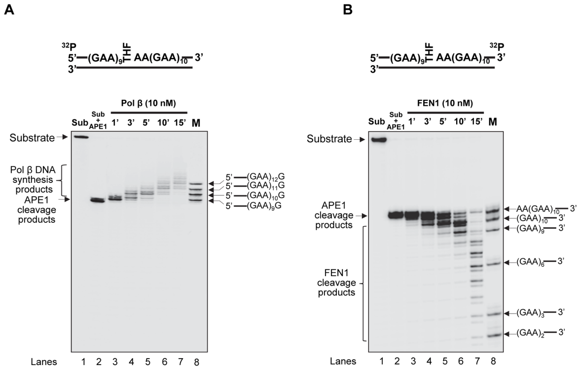
Figure 8. Pol β DNA synthesis and FEN1 cleavage at various time intervals during BER of an abasic lesion in a (GAA) 20 repeat tract. (A) Pol β DNA synthesis during repair of an abasic lesion in the context of (GAA) 20 repeats at different time intervals were conducted as described in the Materials and Methods. The substrate was 32 P-labeled at the 5'-end of the damaged strand. Lane 1 corresponds to the substrate only. Lane 2 corresponds to the substrate that was pre-cut by 50 nM APE1. Lanes 3–7 correspond to reaction mixtures with APE1 pre-cut substrate, 10 nM pol β and 10 nM FEN1 at indicated time intervals. Lane 8 corresponds to synthesized size markers (M). (B) FEN1 cleavage during repair of an abasic lesion in the (GAA) 20 -THF substrate at different time intervals were conducted as described in the Materials and Methods. The substrate was 32 P-labeled at the 3'-end of the damaged strand. Lane 1 corresponds to the substrate only. Lane 2 corresponds to the substrate that was pre-cut by 50 nM APE1. Lanes 3–7 correspond to reaction mixtures with APE1 pre-cut substrate, 10 nM pol β and 10 nM FEN1 at indicated time intervals. Lane 8 corresponds to synthesized size markers (M). The substrate is illustrated schematically above the gel. doi:10.1371/journal.pone.0093464.g008
