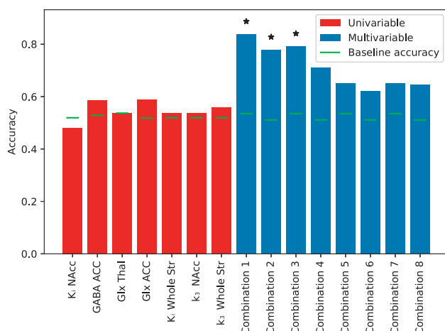
Figure 1. This graph shows the accuracies for prediction of group in univariable and multivariable models, illustrating the predictive accuracy of the tested models. None of the individual neurotransmitter models (red bars) could predict group. Among the multivariable models (blue bars), the best fit model, combination 1, carried out 93.5% of the cumulative model weight (Akaike information criterion controlled for small sample sizes [AICc] = 48.5 and AICc weight = 0.935) and differed from the rest of the models. The variables included in each of the 8 models are provided in Table 3. The dotted green lines indicate balanced accuracy. * indicates significant predictions ( p_{BH} < .05 ). k_3 is the decarboxylation rate (conversion of ^{18}\text{F} -FDOPA to ^{18}\text{F} -dopamine). K_i is the estimate of the dopamine synthesis capacity from the 4-parameter model. ACC, anterior cingulate cortex; ^{18}\text{F} -FDOPA, ^{18}\text{F} -fluorodopa; GABA, gamma-aminobutyric acid; Glx, glutamate plus glutamine; NA CC , nucleus accumbens; Str, striatum; Thal, thalamus.
