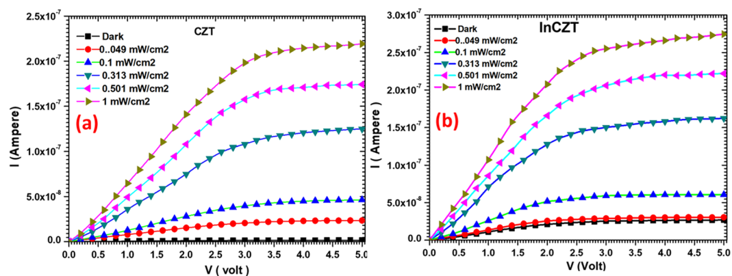
Figure 3. I - V characteristics of (a) CZT and (b) InCZT photodetector devices under different illumination power density.
