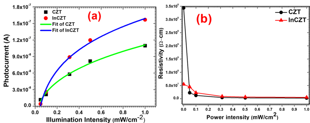
Figure 6. (a) Measured and fitted photocurrent and (b) resistivity of CZT and InCZT crystals under different light illuminations.
