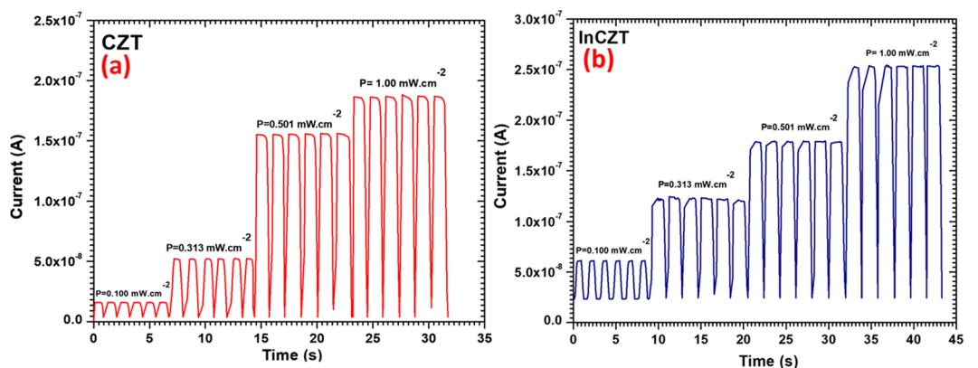
Figure 5. Photo-switching characteristics under different light illumination at 5V bias for (a) CZT and (b) InCZT.
