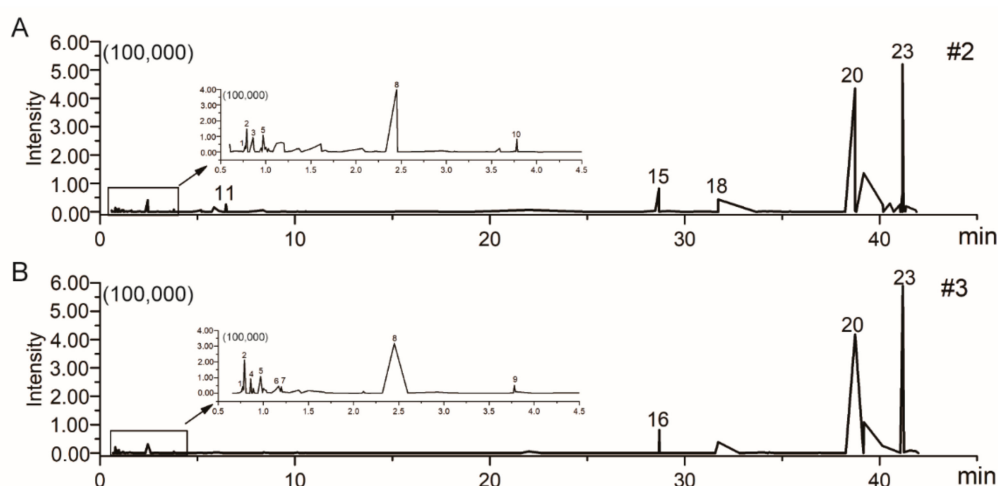
Figure 5. The total ion chromatogram (TIC) of UFLC-Q-TOF-MS/MS obtained from #2 (A) and #3 (B) in the positive-ion mode.
