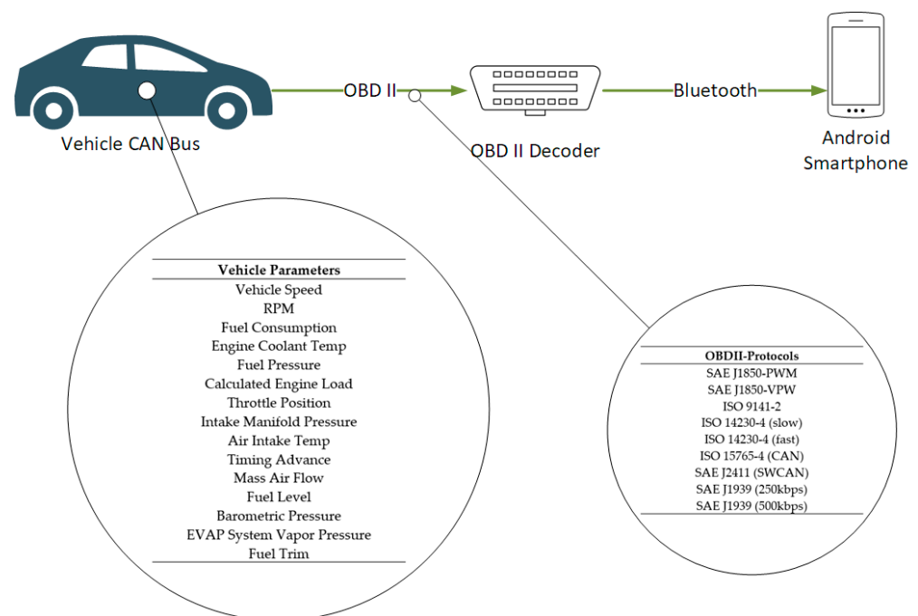
Figure 2. In-car equipment layout.
