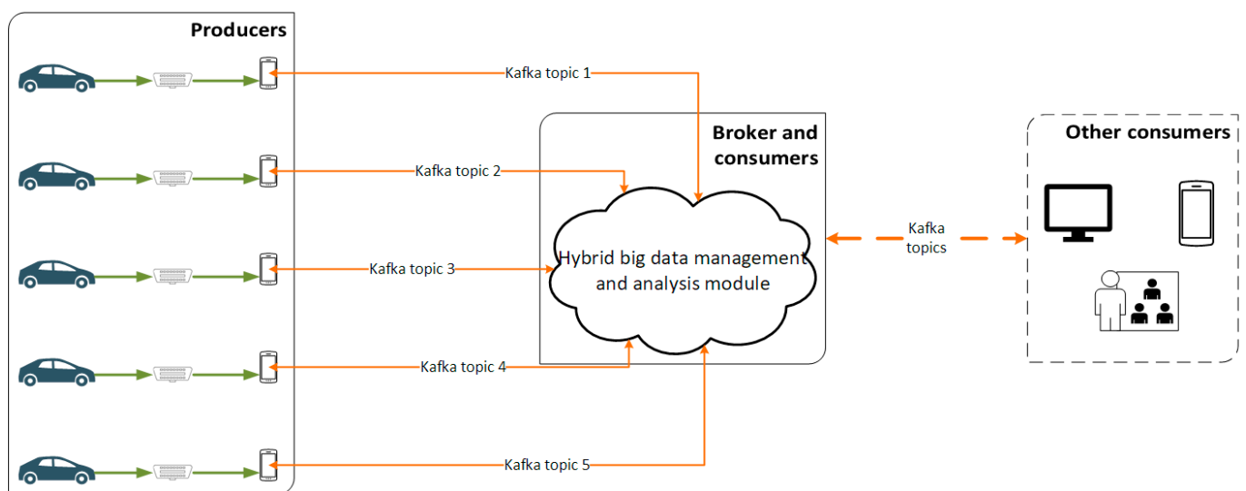
Figure 3. The Kafka streaming process implemented in the present study.
