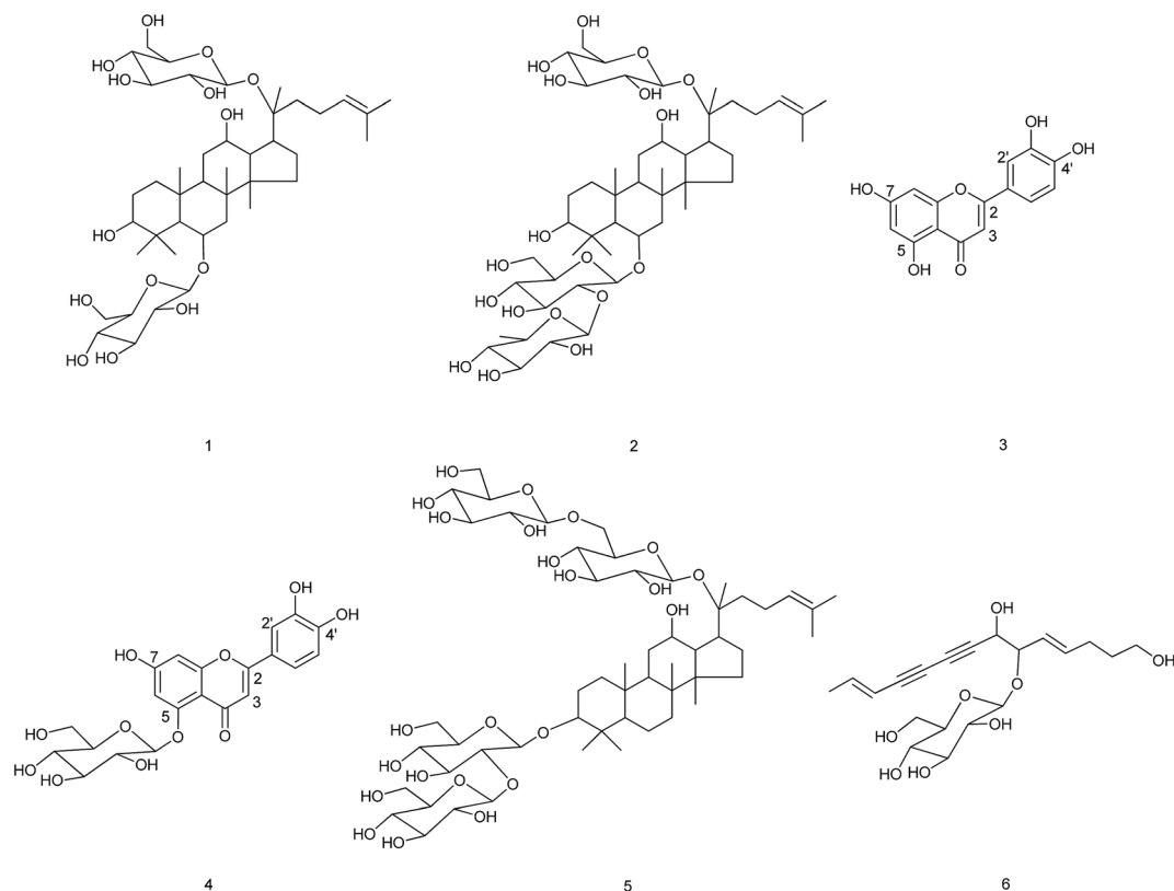
Fig. 2 Compounds isolated from the aerial part of cultivated C. pilosula .
