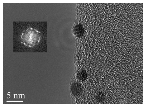
Figure 5. High-resolution TEM image with FFT inset showing the presence of mainly Au(111) lattice planes.
