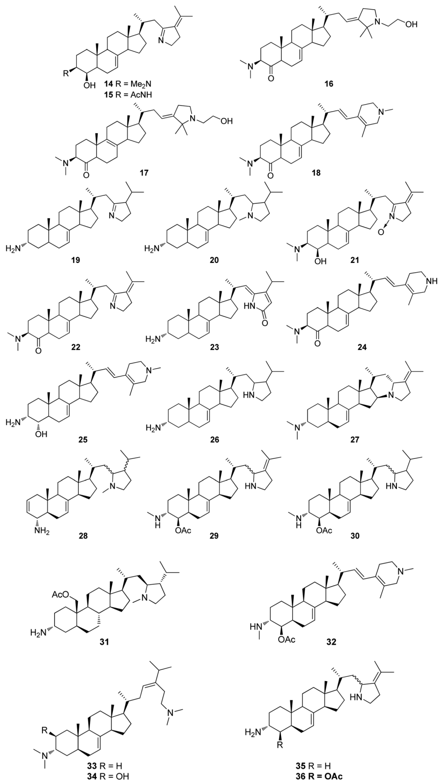
Fig. 3 Reported plakinamines 14–36.
