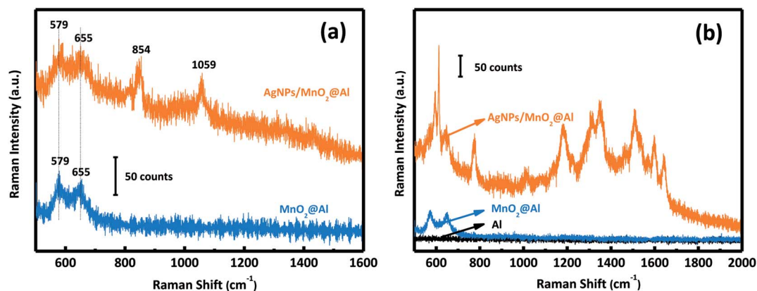
Fig. 5 (a) Raman spectra of MnO 2 @Al and AgNPs/MnO 2 @Al; and (b) SERS activity of Al foil, MnO 2 @Al, and the AgNPs/MnO 2 @Al composite for R6G.
