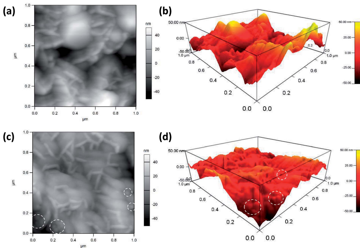
Fig. 4 AFM images of MnO 2 @Al (18 h) before (a), (b) and after (c), (d) deposition of silver colloidal nanoparticles. The white dotted circles show the location of the AgNPs on the MnO 2 @Al substrate.
