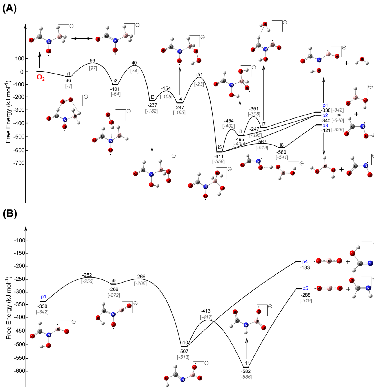
Fig. 6 Potential energy surfaces (PES) for (A) the reaction of N -boryl- N -oxo-formamide [ \text{HCON}(\text{O})\text{BH}_3^- ; BOFA] radical anion with molecular oxygen ( \text{O}_2 ), extending to (B) the formation of boron dioxide ( \text{BO}_2 ) radical. The energy values correspond to the free energies at 298.15 K (black) and 0 K in the parentheses (grey).
