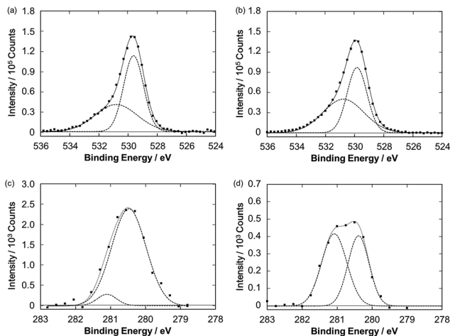
Fig. 7 1s XPS spectra of the Ru–ZnP/TiO 2 /FTO electrodes (a) before and (b) after the PEC operation. Ru 3d_{5/2} XPS spectra of the Ru–ZnP/TiO 2 /FTO electrodes (c) before and (d) after the PEC operation.
