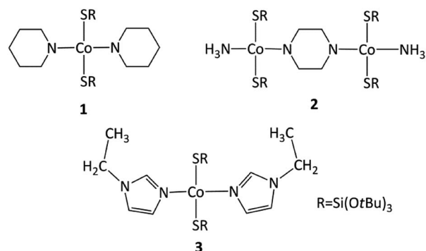
Scheme 1 Synthesized complexes 1–3.
