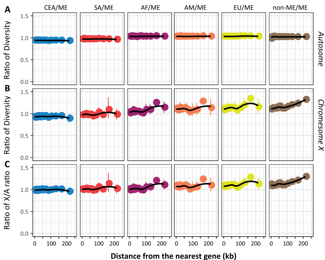
Fig. 6. —Relative nucleotide diversity ( \pi ) and their ratio (X/A) with the physical distance to the nearest gene for the six continental groupings of sheep populations. (A) The ratio of normalized diversity in the groupings of populations from the Middle East (ME) domestication center to those in the other five groupings of populations with the physical distance to the nearest gene for X-linked region. (B) The ratio of normalized diversity in the groupings of populations from the Middle East (ME) domestication to those in the other five groupings of populations with the physical distance to the nearest gene for autosome. (C) Relative X/A diversity in each pair groupings of populations with the physical distance to the nearest gene. 95% confidence intervals from 1,000 bootstrapping iterations are showed in each bin. CEA, Central, and East Asian populations; ME, Middle Eastern populations; SA, South Asian populations; AF, African populations; AM, American populations; EU, European populations. Non-ME, Central and East Asian/South Asian/African/American/European populations.
