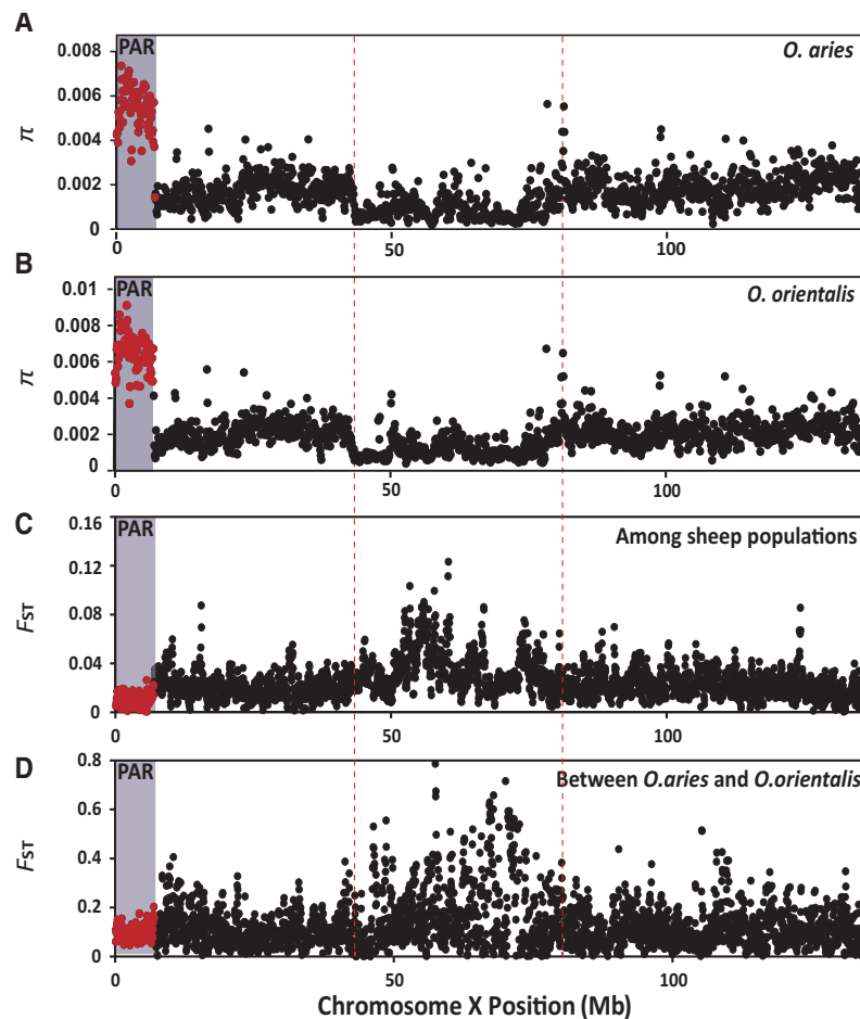
Fig. 2. —Nucleotide diversity and divergence along the X chromosome. (A) Nucleotide diversity ( \pi ) values of domestic sheep ( Ovis aries ) are shown in 50 kb windows and 10 kb steps along chromosome X. (B) Nucleotide diversity ( \pi ) values of Asian mouflon ( O. orientalis ) are shown in 50 kb windows and 10 kb steps along chromosome X. (C) F_{ST} dynamic variation among domestic sheep ( O. aries ) populations are plotted in 100 kb windows and 50 kb steps along chromosome X. (D) F_{ST} dynamic variation between sheep ( O. aries ) and Asian mouflon ( O. orientalis ) are plotted in 100 kb windows and 50 kb steps along the X chromosome. The pseudoautosomal region (PAR) is represented in red dots. A sequential and conserved domain with lower nucleotide diversity and higher divergence is marked by the red dotted lines.
