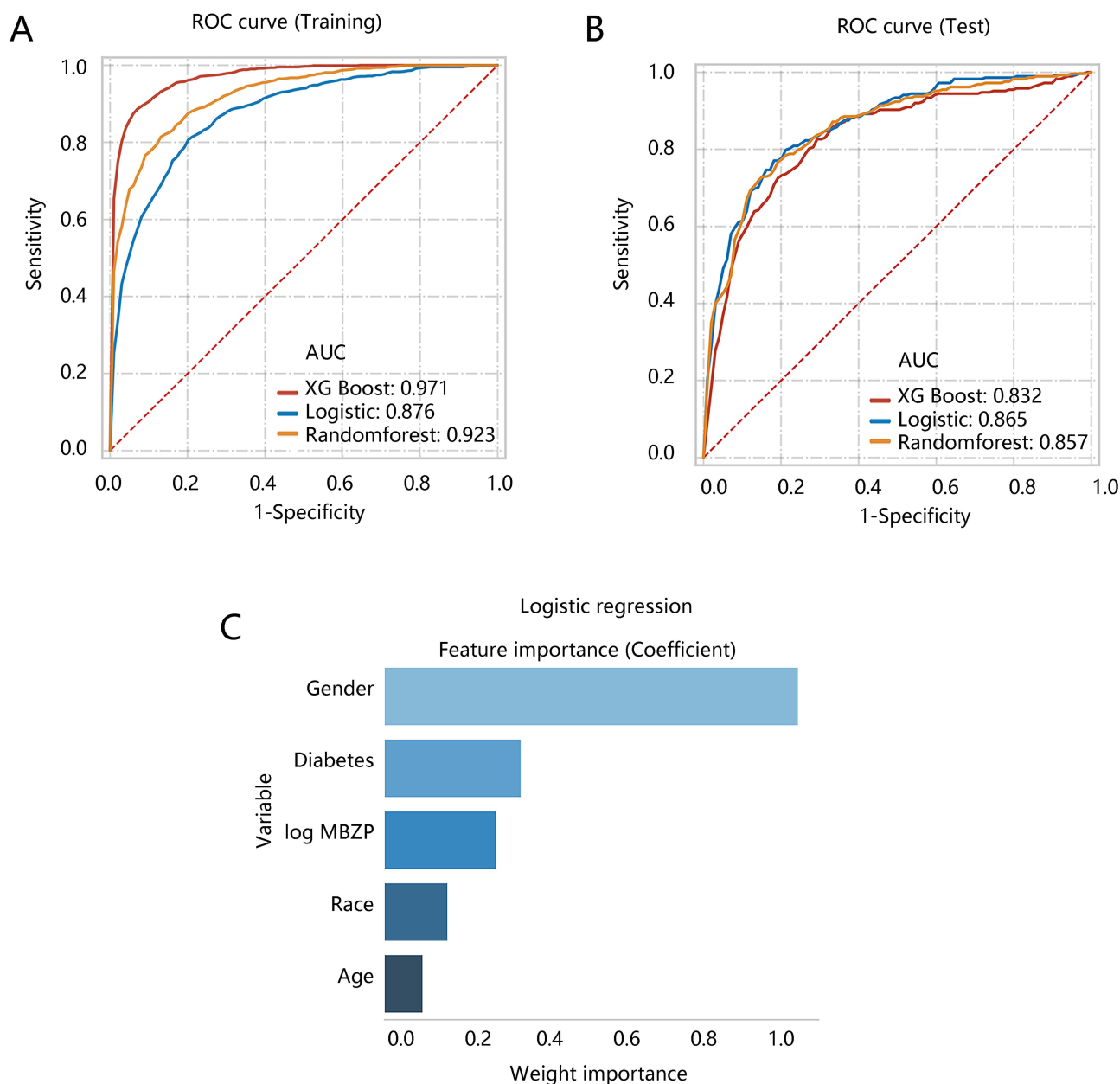
Figure 2 Optimal selection of BMZP-clinical model and feature importance rank. The predictive performance of the MBZP-clinical model for high-frequency hearing loss in the training set (A) and test set (B) to identify logistic regression as the optimal model. (C) The importance of the features in the logistic regression model. Abbreviations: ROC, receiver operating characteristic curve; AUC, the area under the curve.
