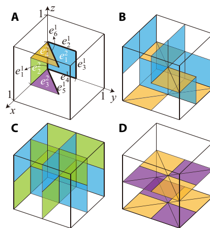
Fig. 2. Topological crystals in space group P4_22_12 (#94). (A) The symmetry-inequivalent 2-cells ( e_{i=1,2,3,4}^2 ) and 1-cells ( e_{i=1,2,3,4,5,6}^1 ) are represented by colored faces and bold lines, respectively. Here, the lattice constants are set to 1, the unit cell is given by 0 < x, y, z < 1 , and the AU is given by 0 < x, y, z < \frac{1}{2} (B to D) The three independent \mathbb{Z}_2 topological crystal generators, where only 2-cells decorated with 2dTIs are shown. (C) and (D) are layer constructions, whereas (B) is not.
