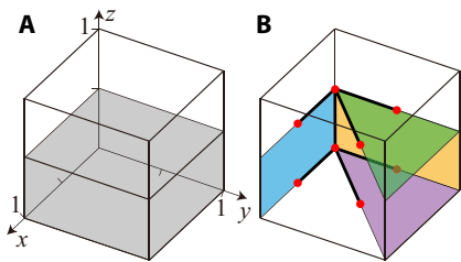
Fig. 1. Cell complex structure for space group P\bar{1} (#2). (A) The AU 0 < x, y < 1 and 0 < z < \frac{1}{2} . (B) The symmetry-inequivalent 2-cells (colored faces), 1-cells (bold lines), and 0-cells (red dots). The other cells can be obtained from these by acting with symmetry operations.
