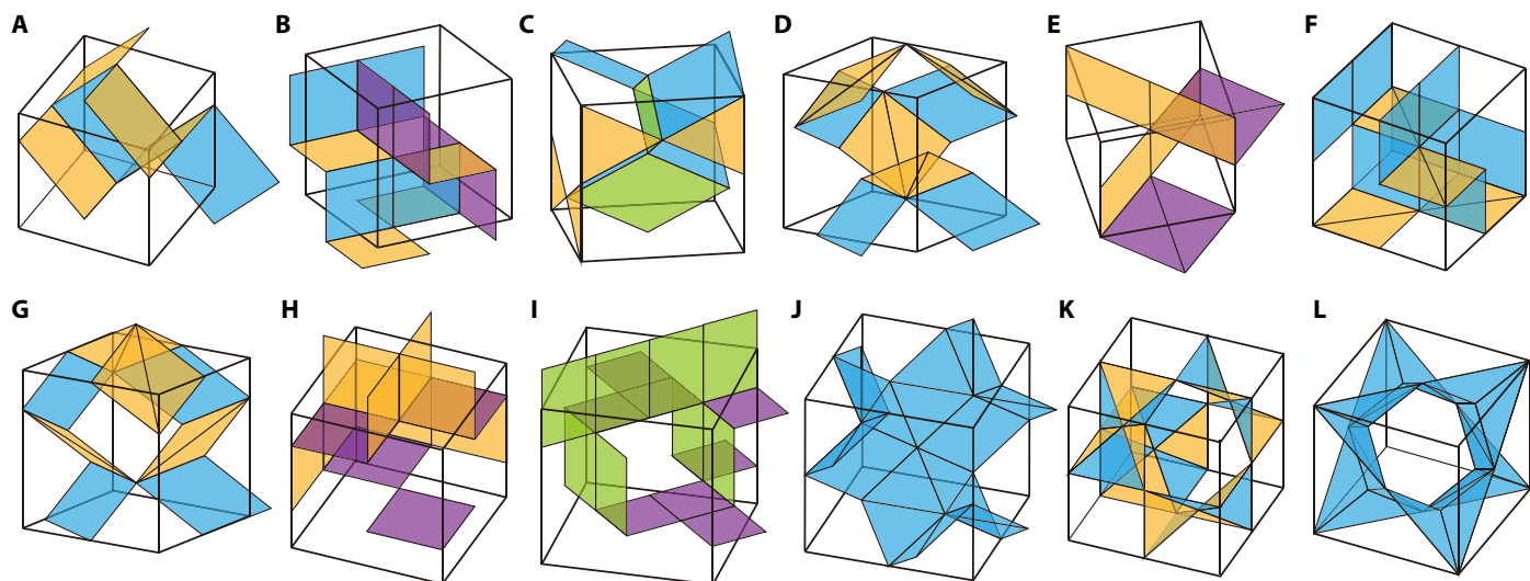
Fig. 3. Illustrations of the topological crystals beyond layer construction. (A) to (L) show these states for space groups Pnn2 (#34), Pnnn (#48), P4_2 (#77), P4_2/n (#86), P4_222 (#93), P4_212 (#94), P4_2cm (#102), P4n2 (#118), P4_2/nnm (#134), Pn\bar{3} (#201), P4_232 (#208), and Pn\bar{3}m (#224), respectively. Inequivalent 2-cells are represented by different colors. The topological invariants of these topological crystals and the coordinates of the plotted 2-cells can be found in the Supplementary Materials.
