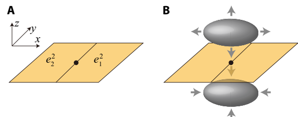
Fig. 4. Illustration of the effects of the equivalence operation in point group \bar{1} without time-reversal symmetry. (A) The 2-cells: e_1^2 : z = 0, x > 0 and e_2^2 : z = 0, x < 0 . (B) The equivalence operation. When a bubble made of 2D Chern insulator with Chern number 1 is created in z > 0 , another Chern bubble with Chern number -1 in z < 0 will be created because of the inversion symmetry. The arrows represent the orientation of the Chern number. We enlarge these two bubbles until they join with the z = 0 plane; then, the Chern number of the state on z = 0 will be subducted by 2.
