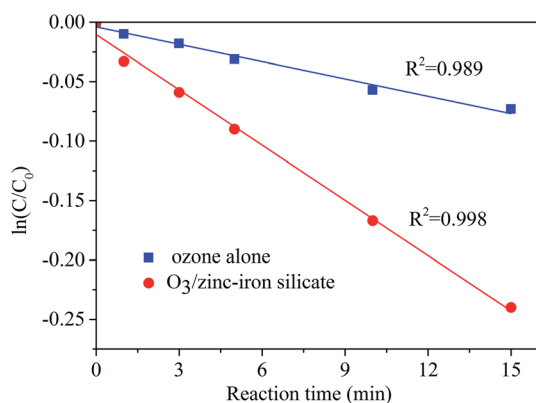
Fig. 9 The decomposition of ozone in the process of \text{O}_3/\text{zinc-iron silicate} process. Ozone dosage: 1.0 \text{ mg} , catalyst dose: 500 \text{ mg} , initial \text{pH} of the ozone solution was adjusted to \text{pH} = 7.0 with \text{NaOH} , reaction temperature 20 \text{ }^\circ\text{C} .
