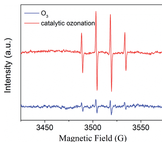
Fig. 10 Spectra of DMPO-OH signals. Ozone dosage: 2.0 \text{ mg L}^{-1} , catalyst dose: 1000 \text{ mg} , initial \text{pH} of the ozone solution was adjusted to \text{pH} = 7.0 with \text{NaOH} , reaction temperature 20 \text{ }^\circ\text{C} , DMPO = 100 \text{ mmol L}^{-1} .
