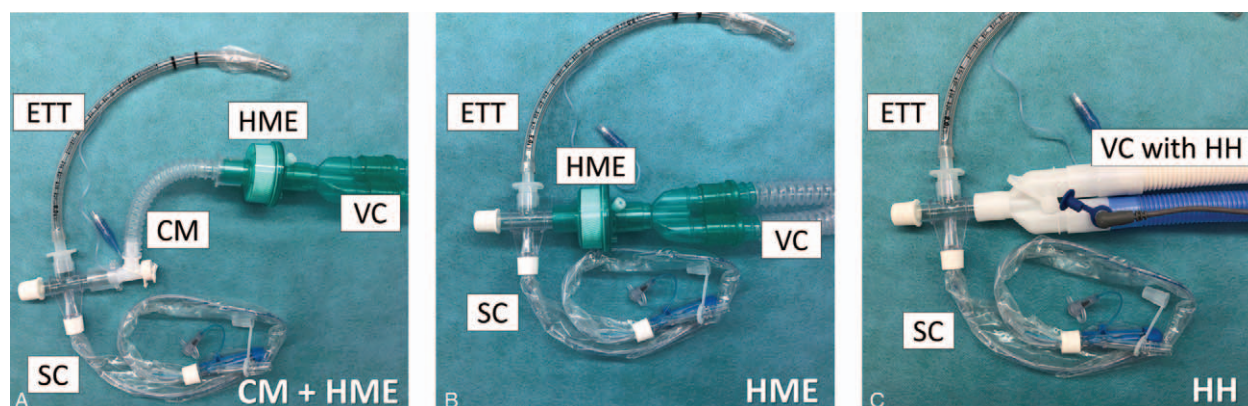
Figure 1. Configuration of the catheter mount and heat-and-moisture exchanger ventilator circuit, heat-and-moisture exchanger ventilator circuit, and head humidifiers. (A): Suction catheter (SC) connected endotracheal tube (ETT), catheter mount (CM), heat-and-moisture exchanger (HME), and ventilator circuit (VC). (B): SC, connected HME and VC. (C): SC and VC connected with heated humidifiers (HH).
