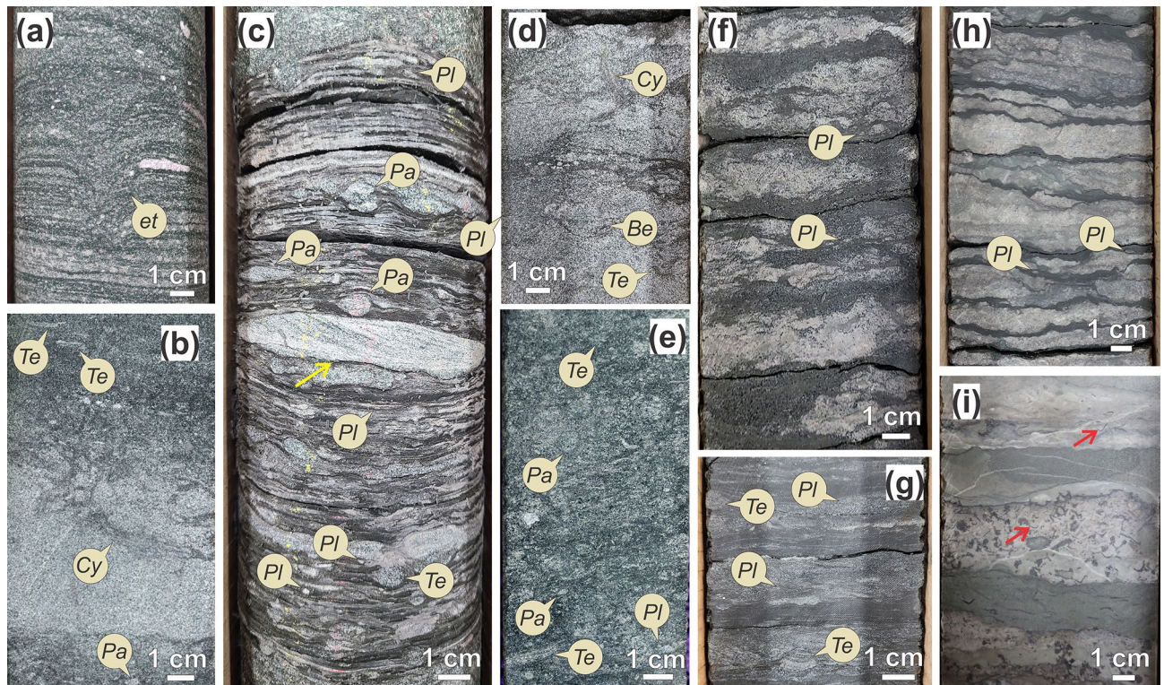
Figure 3. Trace fossils and sedimentary facies of Facies Association 2 (FA2). (a) Escape trace fossil (et) in cross-bedded glauconitic sandstone (Sxgl). (b) Teichichnus rectus and inclined Cylichnus concentricus in interbedded glauconitic sandstone and mudstone (Sgl-Mgl). (c) Parallel-laminated green mudstone (Mg) with very thin-bedded glauconitic sandstone layers and cross-laminated sand lenses (yellow arrow). Teichichnus rectus (Te), Palaeophycus isp. (Pa), and Planolites isp. (Pl). (d) Small Cylichnus concentricus and Bergaueria isp. (Be) in glauconitic sandstone (Sxgl). Scale bar is 1 cm. (e) Moderate to highly bioturbated glauconitic sandstone (Sgl-bio). Teichichnus rectus (Te), Palaeophycus isp. (Pa), and Planolites isp. (Pl). (f) Interbedded glauconitic sandstone and limestone (Sgl-Lst) with Planolites isp. (Pl). (g) Teichichnus rectus (Te) and Planolites isp. (Pl) in interbedded glauconitic sandstone and mudstone (Sgl-Mgl). Note the presence of discrete thin intervals with undetermined bioturbation mottling. (h) Interbedded mudstone and limestone (M-Lst). (i) Limestone with discontinuous mudstone and trilobite and linguliform brachiopod fragments (red arrows). Photographs taken by A.I. Labels created by A.I. using CoreDRAW 2017 v.19.1.0.419 software.
