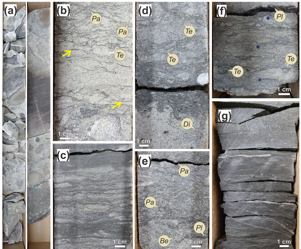
Figure 2. Trace fossils and sedimentary facies of Facies Association 1 (FA1). (a) General view of granule to boulder conglomerate (Cg). Core width 7.5 cm. (b) Teichichnus rectus ( Te ) and Palaeophycus isp. ( Pa ) in interbedded sandstone and conglomerate (S-Cg). Sandstone bed is mudstone draped (yellow arrows) forming flaser and wavy bedding. (c) Argillaceous sandstone and mudstone (Sd). (d) Teichichnus rectus ( Te ) and poorly defined Diplocraterion isp. ( Di ) penetrating in bioturbated gravelly sandstone (Sg-bio). (e) Palaeophycus isp. ( Pa ) and Planolites isp. ( Pl ) in bioturbated gravelly sandstone (Sg-Bio). Bergaueria isp. ( Be ) preserved at base of sandstone layer. (f) Teichichnus rectus ( Te ) and Planolites isp. ( Pl ) in argillaceous sandstone and mudstone (Sd). (g) Parallel-laminated shale (Sh). Photographs taken by A.I. Labels created by A.I. using CoreIDRAW 2017 v.19.1.0.419 software.
