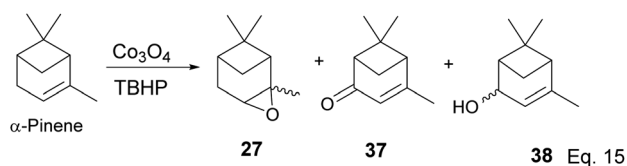
Scheme 12 Cobalt oxide-promoted transformation of \alpha -pinene.
