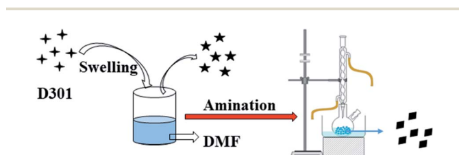
Scheme 1 Flowcharts for the D301 resin modification reaction.
