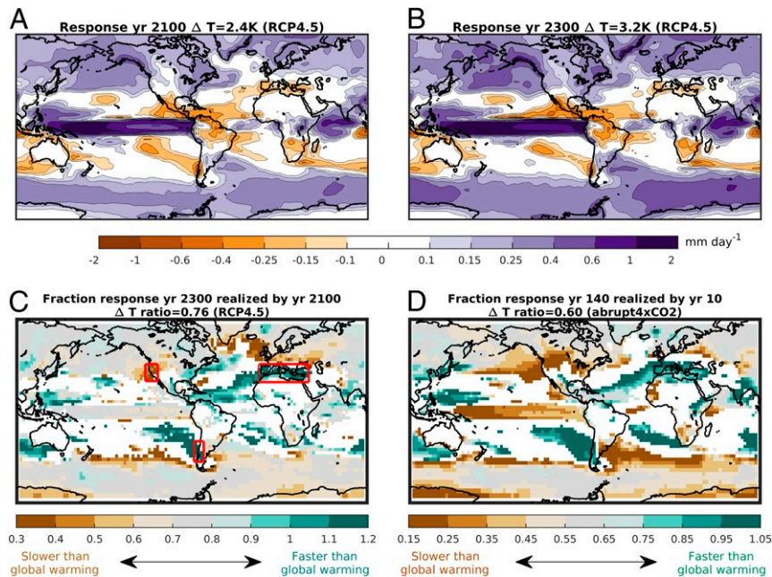
Fig. 1. (A) CMIP5 multimodel mean annual-mean precipitation response ( \text{mm}\cdot\text{d}^{-1} ) by year 2060 to 2099 in the RCP4.5 scenario relative to 1900 to 1949. (B) As in A, but for the long-term precipitation response by year 2260 to 2299. In the titles, \Delta T indicates the global warming realized in each period. (C) Ratio of A to B, i.e., the fraction of the long-term response already realized by 2060 to 2099. Gray shading implies that the ratio in the precipitation response scales like global-mean warming. Brown (green) shading implies that the precipitation response is slower (faster) than global warming. White shading shows where less than 75% of models agree on the direction of change. (D) As in C, but for the fraction of the mean response in the abrupt4xCO2 experiment in years 120 to 139 that is already realized by years 5 to 10. The multimodel means are based on all of the CMIP5 models available for each experiment (SI Appendix, Table S1). The results in D are confirmed both in the subset of seven CMIP5 models that form the basis of this study (SI Appendix, Fig. S1A) and in an alternative calculation where the rapid adjustment is explicitly accounted for (SI Appendix, Fig. S1B). The red boxes in C show the domains of the area-averaged values in Table 1.
