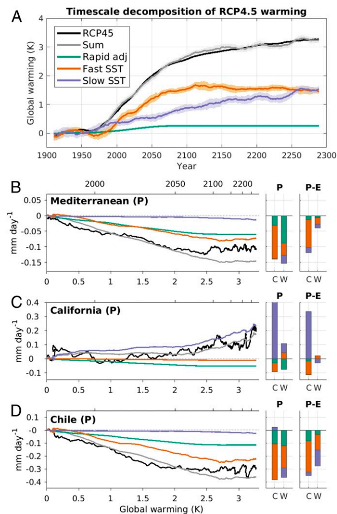
Fig. 4. (A) Multimodel mean contribution of the rapid adjustment and of the fast and slow SST-driven responses to the global-mean warming in the RCP4.5 scenario. (B–D) Decomposition of the annual-mean precipitation changes over land in the Mediterranean (B), California (C), and Chile (D) in RCP4.5 in terms of the three timescales of response. In B–D, the time evolution of the response is presented against global-mean warming. The equivalent years are indicated on the upper axis. B–D, Right show the timescale contributions to the P and P - E seasonal-mean responses in 2250 to 2299 (C for cold season, W for warm season). These are presented as stacked bars, in which the amplitude of the contribution is given by the length of the bar, separately for the positive and negative values. All time series have been filtered with a 21-y running mean. The shading in A represents a 95% CI based on the variability within each 21-y window.
