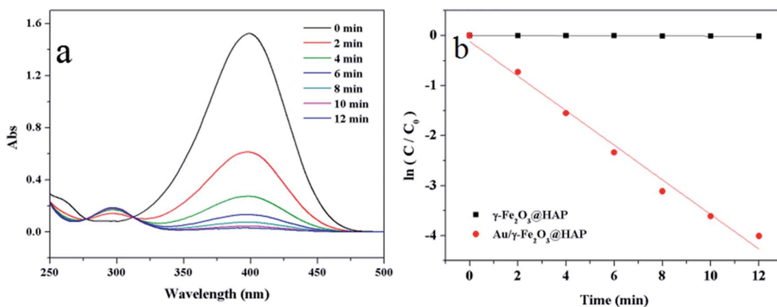
Fig. 6 (a) UV-Vis spectra for the catalytic reduction of 4-NP solution catalyzed by Au/ \gamma -Fe 2 O 3 @HAP-2, (b) plots of \ln(C/C_0) versus reaction time catalyzed by Au/ \gamma -Fe 2 O 3 @HAP-2 and \gamma -Fe 2 O 3 @HAP. Reaction conditions: Au/ \gamma -Fe 2 O 3 @HAP-2 or \gamma -Fe 2 O 3 @HAP (2 mg), 4-NP solution (10 mL, 1 mmol L -1 ), NaBH 4 solution (15 mL, 0.067 mol L -1 ) at 293 K.
