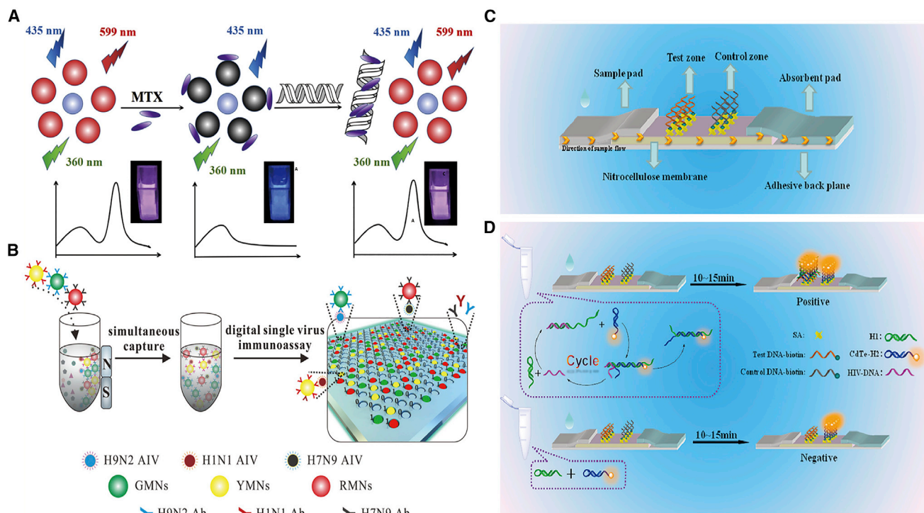
Figure 3. Schematic Diagrams of Different QDs-Based Biosensing Nanoplatforams for Virus Detection
