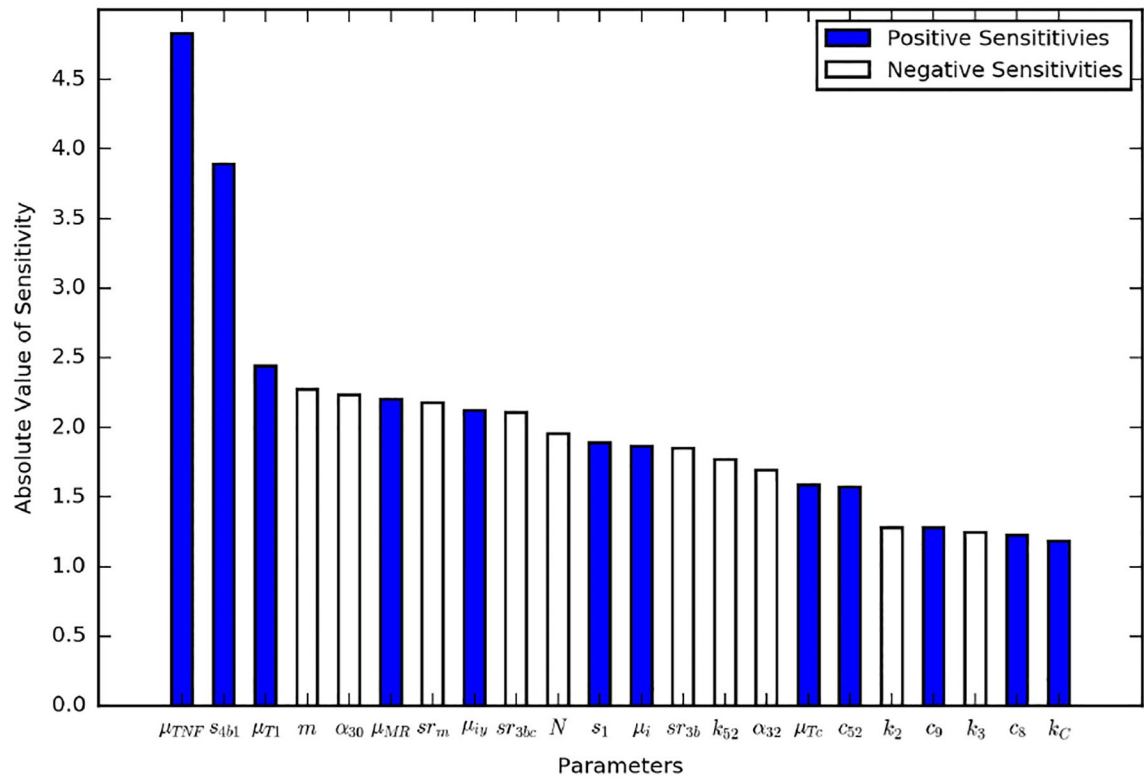
Figure 5. Local sensitivity analysis results for the parameters from the immune response model that were at least as sensitive as the new model parameter k_C .
