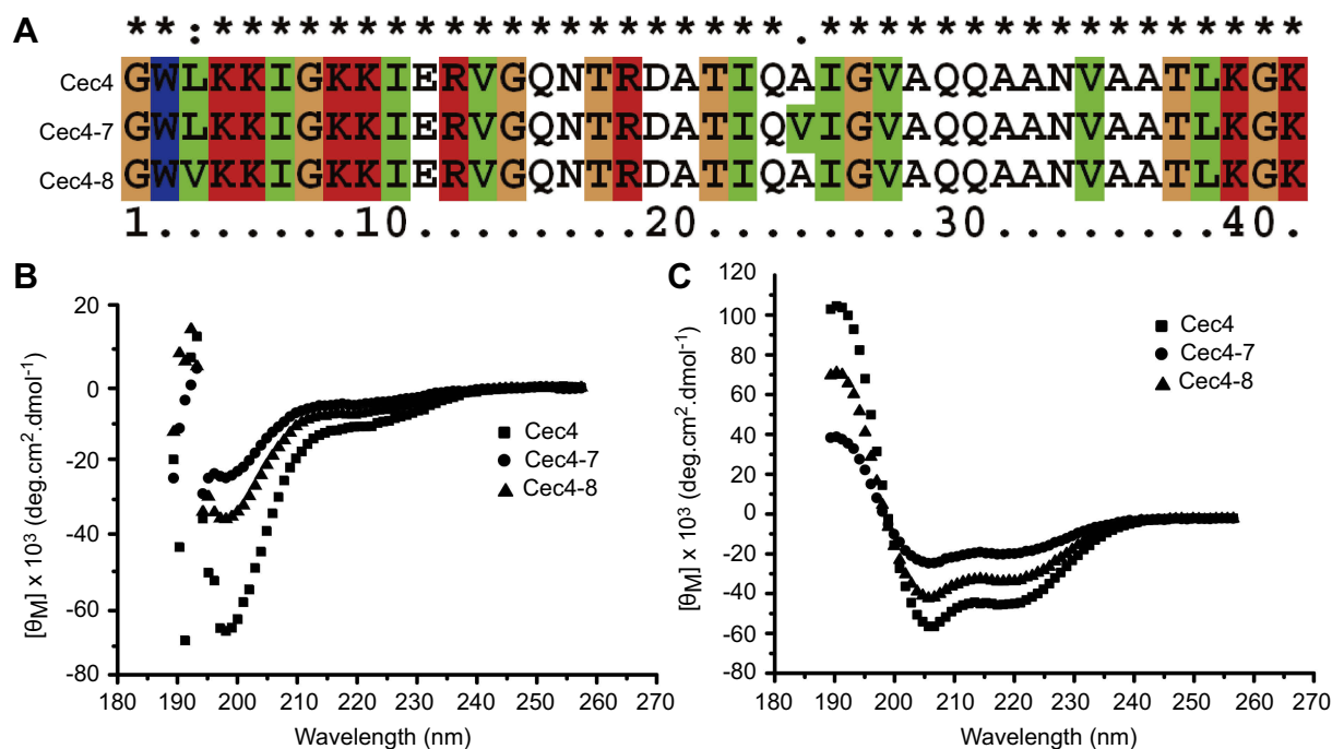
Figure 1 Sequence alignment and circular dichroism (CD) spectra of peptides. (A) Multi-sequence alignment of peptides performed using ClustalW ( http://embnet.vital-it.ch/software/ClustalW.html ). CD spectra of Cec4, Cec4-7, and Cec4-8 in PBS (B) and the microbial membrane-mimicking environment (25 mM SDS micelles solution) (C).
