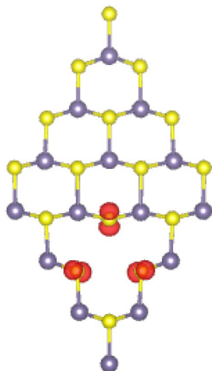
Fig. 5 Spin surface (iso-surface value: 0.01 \text{ e } \text{Å}^{-3} ) in GeS monolayer with a single Ge vacancy.
