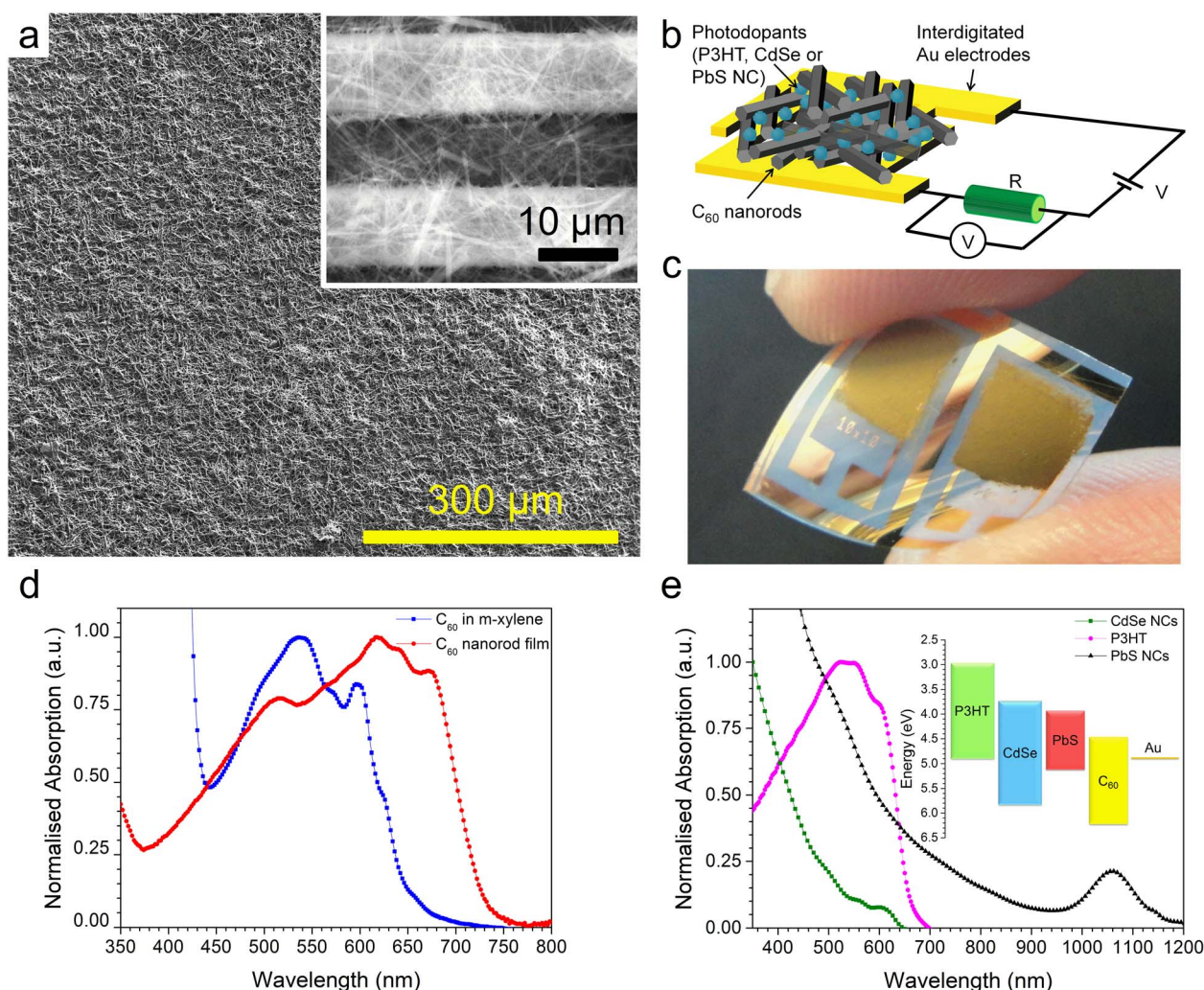
Figure 2 | C_{60} nanorod photoconductor device architecture and absorption. (a) A 5 kV SEM image of a typical C_{60} nanorod photoconductor fabricated via depositing a C_{60} nanorod film onto pre-patterned interdigitated Au electrodes. Inset to (a) is a 30 kV SEM image showing C_{60} nanorods bridging 10 \mu\text{m} wide interdigitated electrodes with an inter-electrode spacing of 10 \mu\text{m} . (b) A schematic depicting the planar device architecture employed for fabricating photoconductor devices and the electrical circuit diagram used to characterize the devices. (c) Photograph of two typical C_{60} nanorod photoconductor devices fabricated on a flexible PEN substrate. The active area covers the region of interdigitated electrodes which measures 5 \times 5 mm. (d) Normalised optical absorption spectra of C_{60} dissolved in m-xylene and a C_{60} nanorod film. C_{60} nanorods display broadened and extended absorption, red shifted by \sim 100 nm, compared to C_{60} in solution. (e) Normalised optical absorption spectra of P3HT, CdSe NCs, and PbS NCs used for photodoping the C_{60} nanorod devices. Inset to (e) is a schematic of the relative energy level alignment between C_{60} and the photodopants. The relative energy level alignment strongly favours photoexcited electron transfer from the photodopants to the C_{60} with holes remaining trapped in the photodopant.
