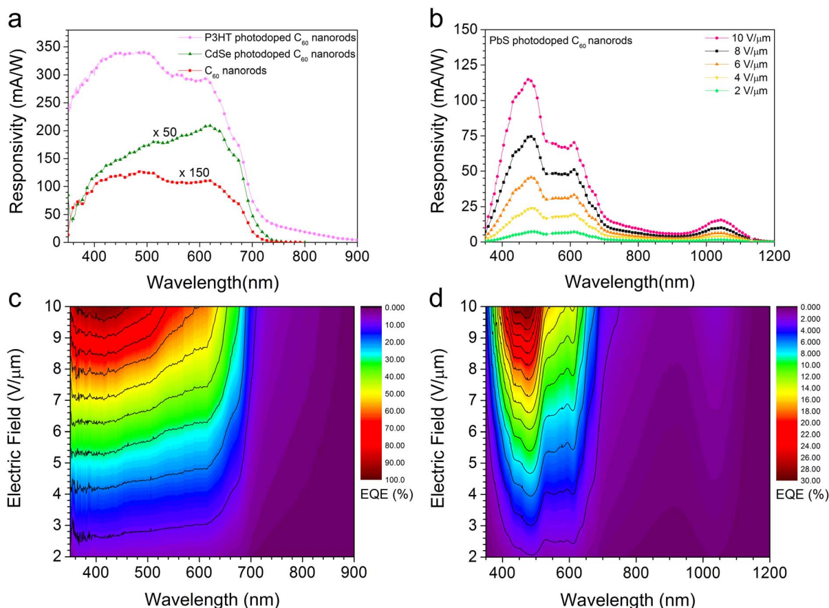
Figure 3 | Spectral responsivity and external quantum efficiency of C 60 nanorod photoconductor devices. (a) Relative comparison of spectral responsivity obtained for C 60 nanorod only and P3HT or CdSe NC photodoped C 60 nanorod devices. Responsivity was measured using an applied electric field of 10 V/μm -1 , and a modulation frequency of 235 Hz. All devices display photosensitivity across the full visible spectrum with the photodoping significantly enhancing the responsivity by up to 2 orders of magnitude. (b) Electric field dependent spectral responsivity of PbS NC photodoped device. The responsivity spectrum follows the C 60 absorption spectrum in the visible region, confirming that the ultralow photodoping provided via PbS NCs enhances the photosensitivity of C 60 nanorods. The spectral responsivity is extended by the use of PbS NC to provide UV-vis-NIR sensitivity. (c) The EQE of a P3HT photodoped device as a function of applied electric field and wavelength displaying a peak EQE approaching ~100% at 415 nm. (d) The EQE of a PbS NC photodoped device as a function of applied electric field and wavelength. It can be seen that EQE of the device is strongly field dependent in the region where the C 60 nanorods absorb (350–750 nm) whilst in spectral range (750–1150 nm) the EQE remains below ~2%, even with increase in the applied electric field.
