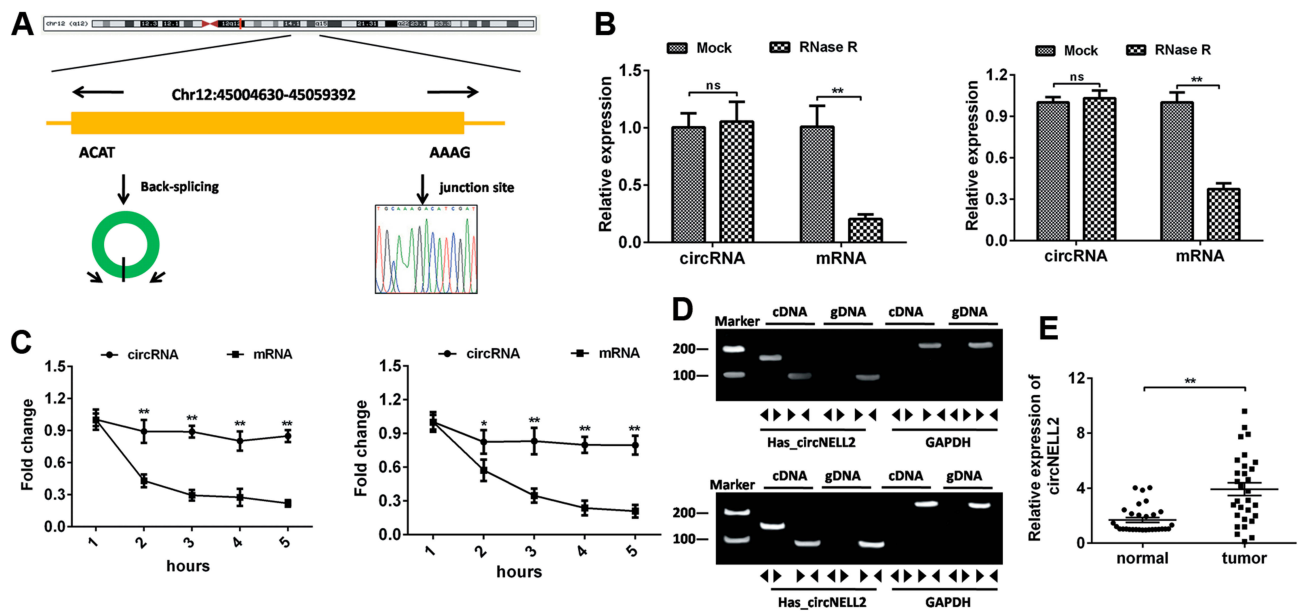
Figure 1 The identification of circNELL2. (A) circNELL2 was back-spliced by exon 14 and exon 15 of the neural EGFL like 2 (NELL2) gene with the length of 294 nucleotides. The existence of circNELL2 were confirmed by sanger sequencing, the arrow shows the head-to-tail splicing junction site of circNELL2. (B) After RNase R treatment, the expression of linear RPL13 mRNA and circNELL2 were detected using qPCR. (C) qRT-PCR analysis of RPL13 mRNA and circNELL2 in cardiomyocytes after treatment with Actinomycin D for 1, 2, 3, 4, 5 h, respectively. (D) The existence of circNELL2 was validated by RT-PCR. Divergent primers amplified circNELL2 in cDNA but not genomic DNA (gDNA). (E) qPCR was performed to evaluate the expression of circNELL2 in ESCC tissues. *P< 0.05, **P< 0.01.
