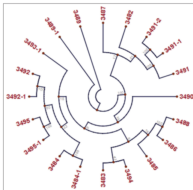
Figure 2: Analysis of MLST 20 Isolated Iranian Helicobacter pylori . Phylogenetic tree using neighbor-joining-tree algorithm in software Viewer 8 CLC Sequence been plotted
