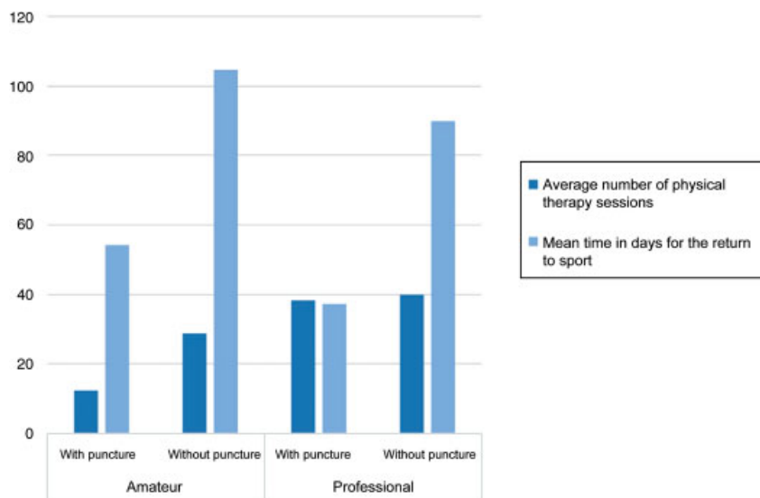
Fig. 3 Amateur (left) and professional athletes (right) groups. The intervention is evaluated among amateur and professional athletes and confronted with the control group through the following variables: average number of physical therapy sessions and mean time, in days, for the return to sport.
