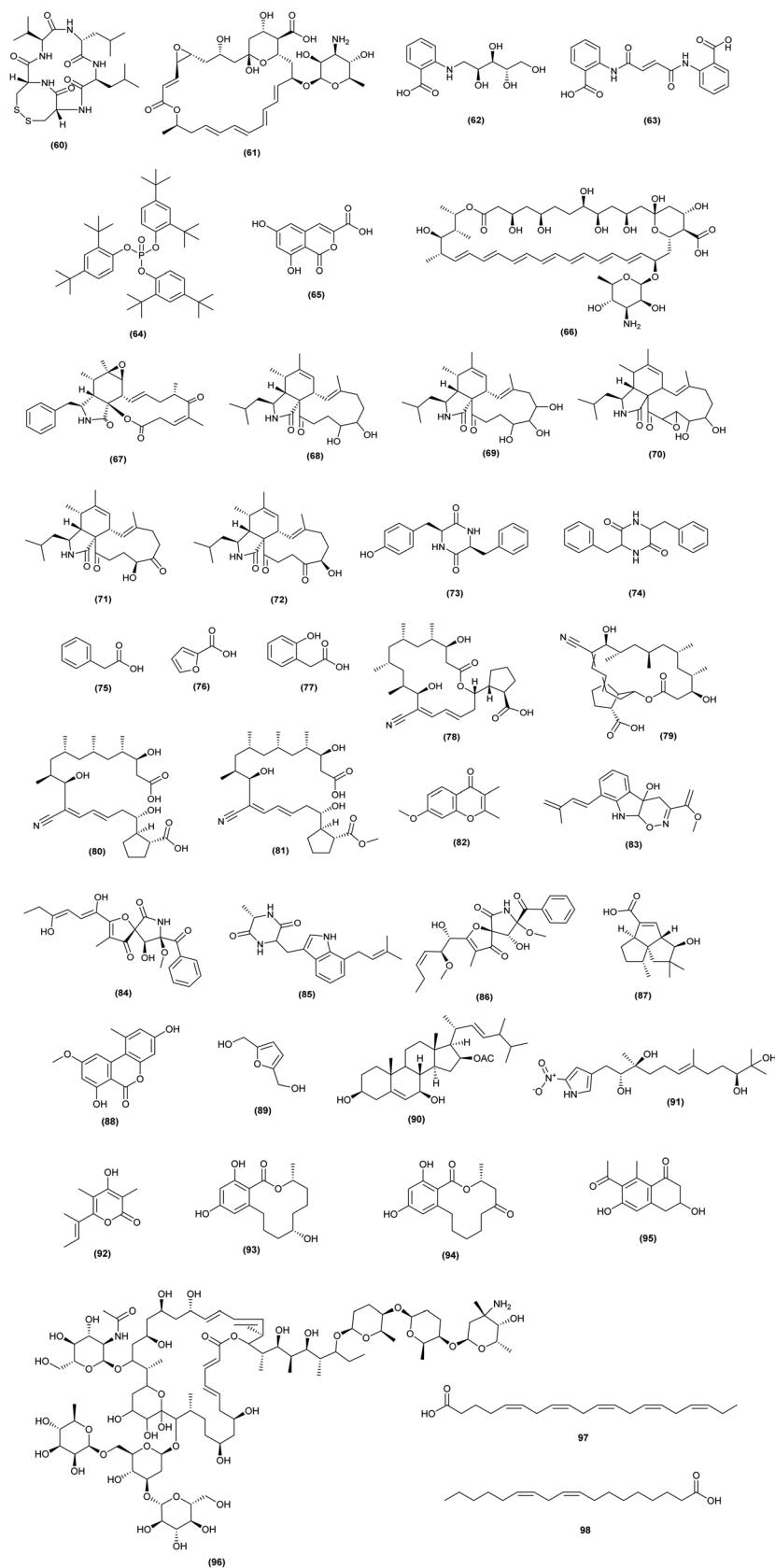
Fig. 4 Chemical structures of compounds 60–96 reported upon co-cultivation of actinomycetes with fungi. Cytochalasins: rosellichalasin (67), 19,20-dihydro-aspochalasin D (68), aspochalasin E (69), aspochalasin H (70), aspochalasin M (71), aspochalasin P (72); chemical structures of compounds 97 and 98 reported upon co-cultivation of actinomycetes with alga. The configuration of all stereocenters in each compound is shown as given in the literature.
