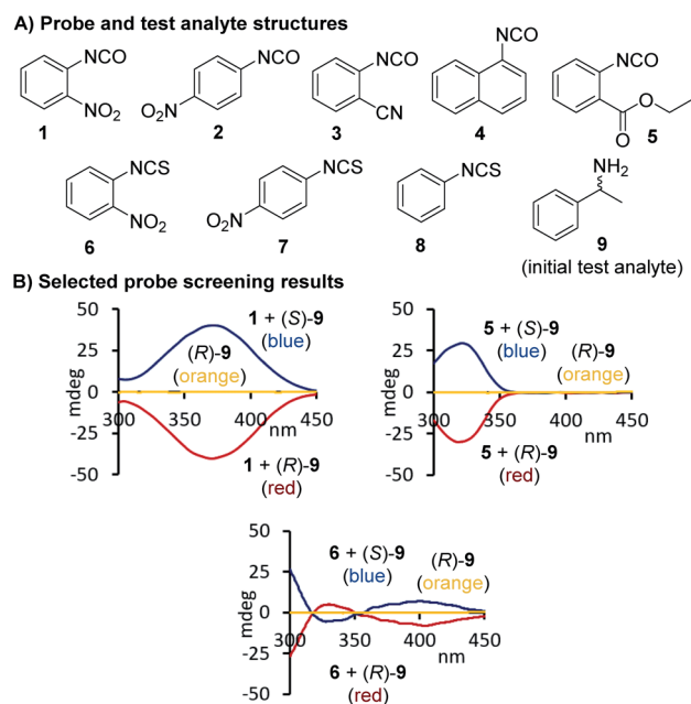
Fig. 1 Structures of arylisocyanate and arylisothiocyanates 1–8 and comparison of the chiroptical responses of 1 , 5 , and 6 to the enantiomers of 1-phenylethylamine. The CD spectrum obtained with free ( R )- 9 under the same conditions but in the absence of an iso(thio) cyanate probe is shown in orange. Conditions: 1-phenylethylamine (82.5 mM) and an iso(thio)cyanate probe (99.0 mM) were mixed in 1.0 mL of \text{CHCl}_3 and the reaction was stirred overnight followed by dilution with acetonitrile to 0.37–0.50 mM prior to CD analysis, see ESI† for details.
