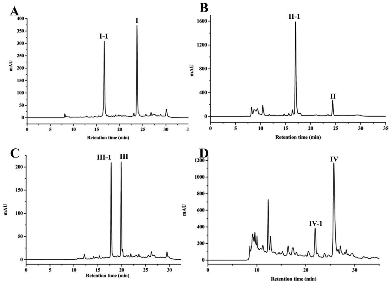
Fig. 1 HPLC chromatograms of biotransformation of (A) 7-hydroxy-4,8-dimethylcoumarin (I), (B) 6-hydroxy-4,7-dimethylcoumarin (II), (C) 6,7-dihydroxy-4-methylcoumarin (III), (D) 5-hydroxy-4,7-dimethylcoumarin (IV). Substrates I, II, III and IV could be transformed into I-1, II-1, III-1 and IV-1 by C. acuminata CMCs, respectively.
