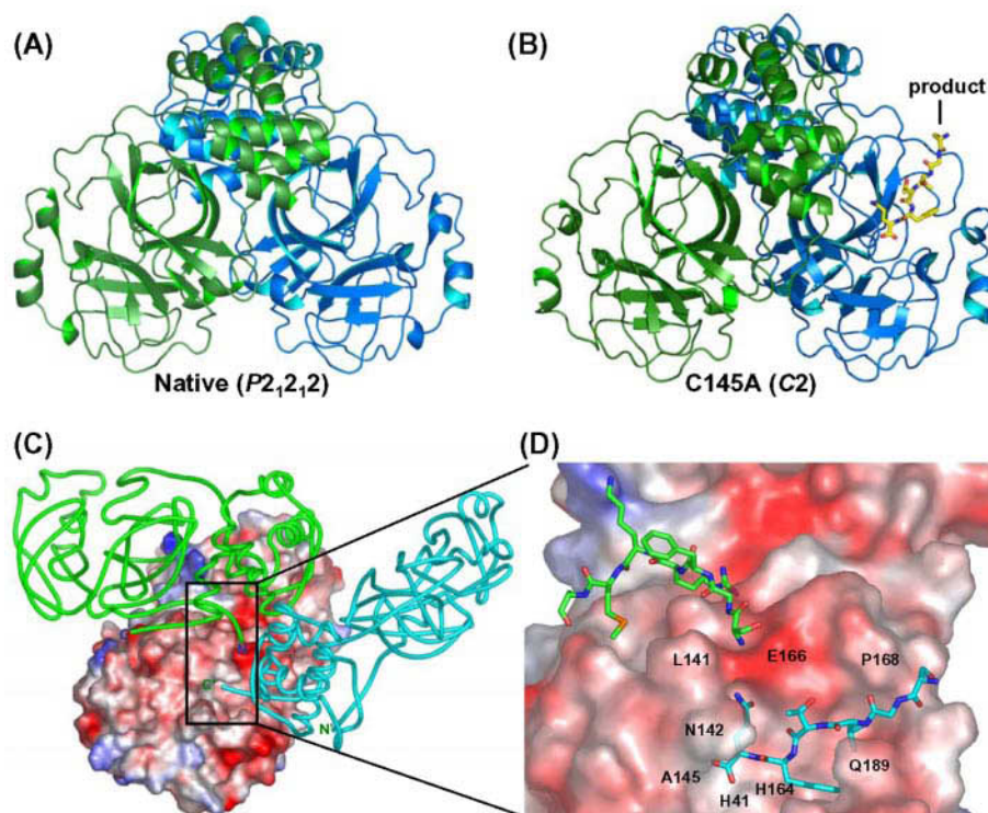
FIG. 1. Crystal structures of the wild-type and C145 mutant 3CL pro . In A and B, the overall three-dimensional structures of wild-type and C145A mutant 3CL pro are shown as ribbons (protomer A is green and protomer B is blue), and the “product” in the active site cleft between domain I and II is shown in yellow. In C, the dimer structure is composed of protomer A (shown with a solid tube in green) and protomer B (shown with charge potentials). The C terminus of protomer B' (shown in cyan) in another asymmetric unit is intercalated into the active site of protomer B. D, an enlarged view of C near the active site, showing the C-terminal amino acids of protomer B' as well as the N-terminal amino acids of protomer A in the neighborhood of the active site of protomer B.
