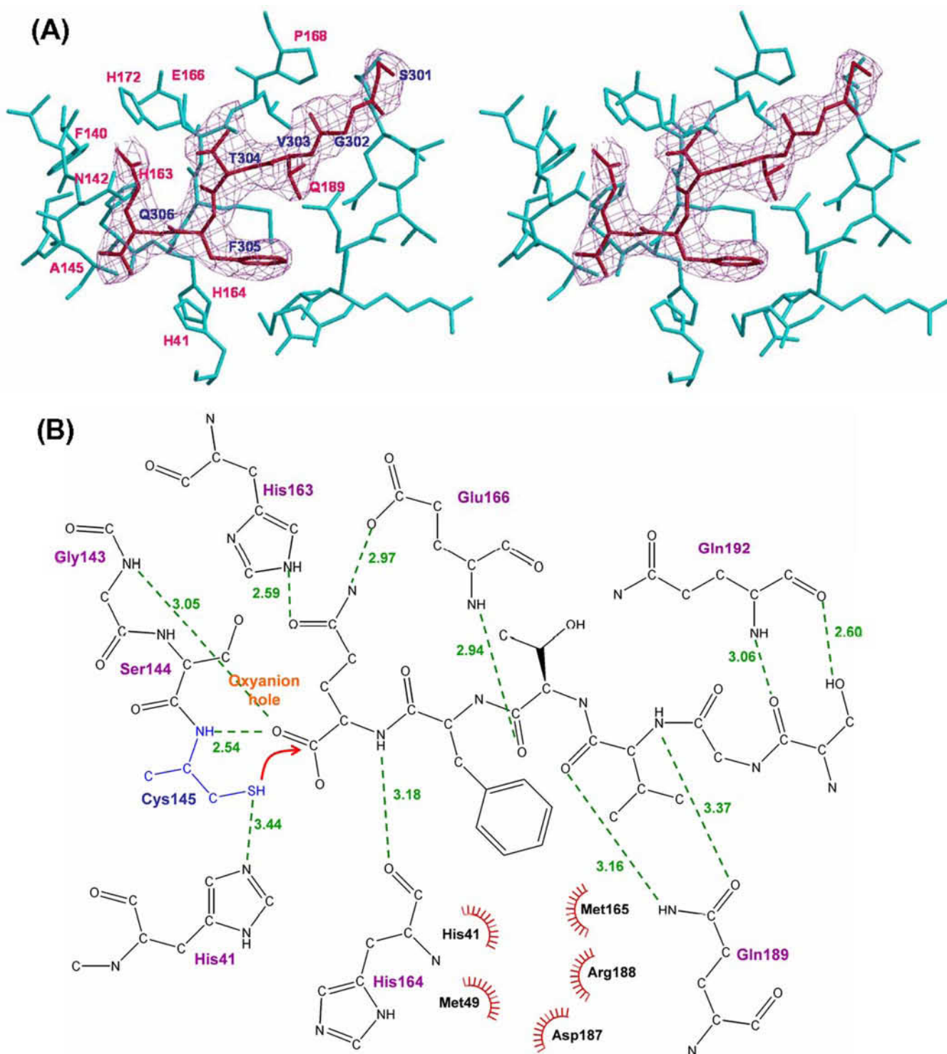
FIG. 5. Molecular interactions of the active site residues of protomer B with the C-terminal residues of protomer B'. A, stereo view of the electron density map of the C-terminal region (red stick) of protomer B' bound in the S pockets (cyan stick) of protomer B. B, details of the molecular interactions between the active site S1-S6 pockets of protomer B and the C-terminal residues of protomer B'. H-bonds are shown as green broken lines.
